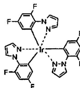
\text{Ir(dfppz)}_3
