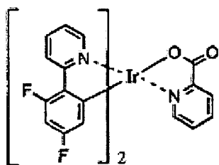
\text{F}_2\text{Irpic}
