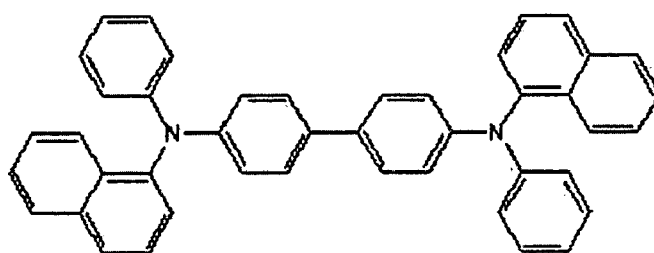
NPB
