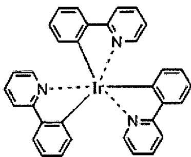
\text{Ir(ppy)}_3
