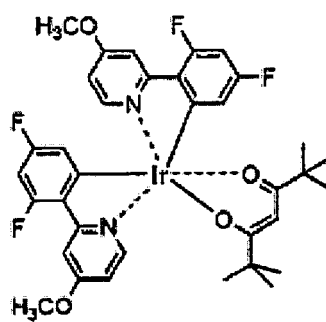
(\text{F}_2\text{ppy})_2\text{Ir(tmd)}
