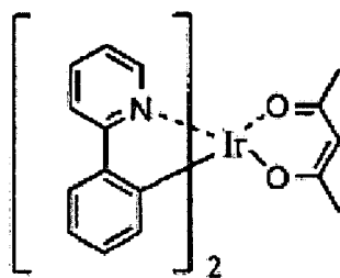
\text{Ir(ppy)}_2(\text{acac})
