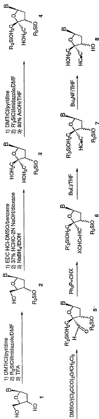
Scheme 1. Synthesis of 4'-ethynyl-2'-deoxynucleosides from 2'-deoxynucleosides
