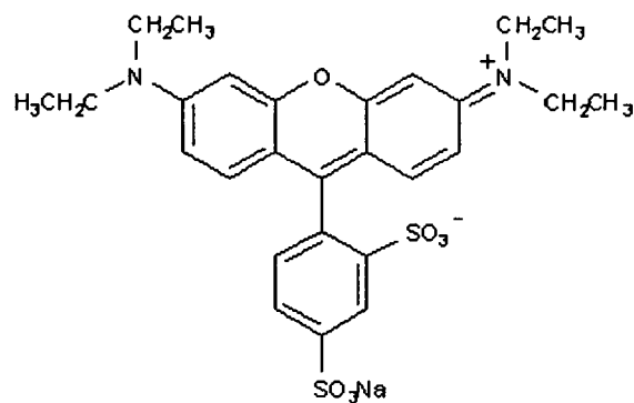
C.I. Acid Red 52
