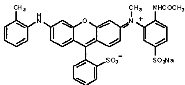
Comparative Colorant Compound (3)
