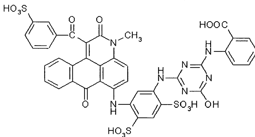
Combined-Use Colorant Compound (4)
