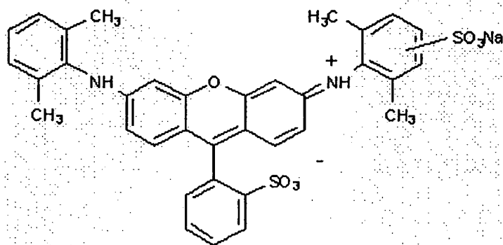
C.I. Acid Red 289
