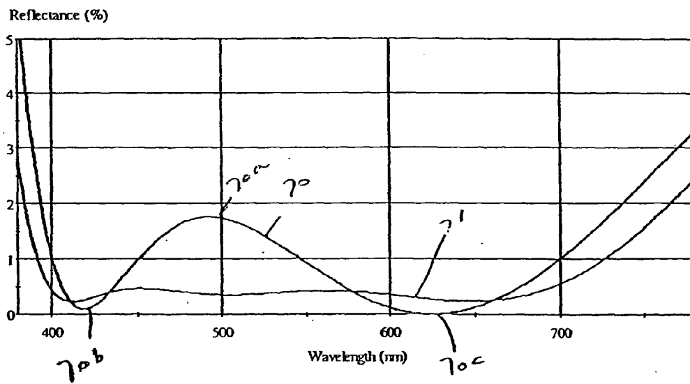
Conventional Anti-Reflective Vs NRC
