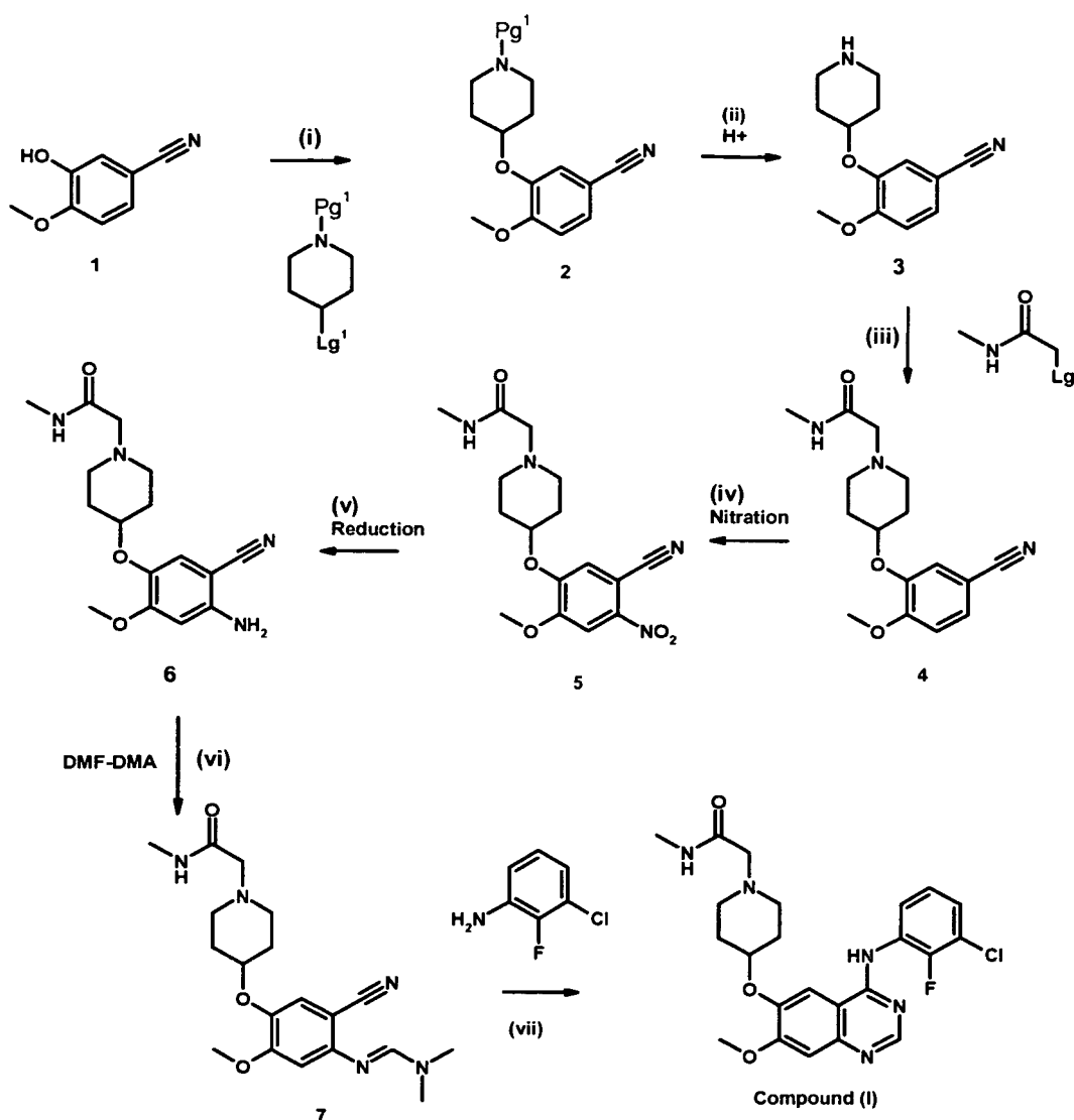
Reaction Scheme 1
