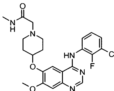
Compound (I)
