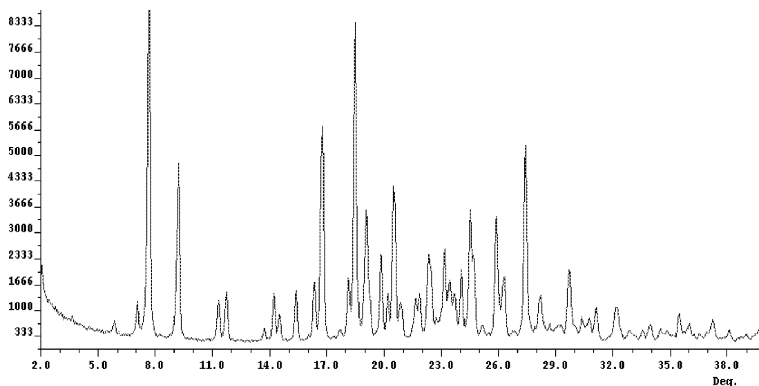
Fig.6: An X-ray powder diffraction pattern of crystalline pemetrexed diacid characterized by an X-ray powder diffraction pattern with peaks at about 7.7, 9.2, 16.7, and 27.4 degrees two-theta \pm 0.2 degrees two-theta.
