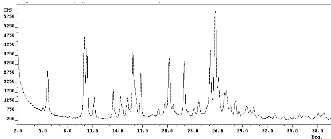
Fig. 1: An X-ray powder diffraction pattern of crystalline pemetrexed diacid characterized by an X-ray powder diffraction pattern with peaks at about 10.0, 10.3, 22.0 and 25.7 degrees two-theta \pm 0.2 degrees two-theta.
