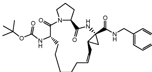
Compound 2307
