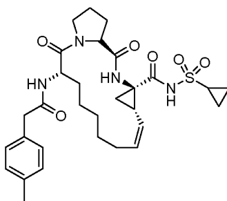
Compound 2140
