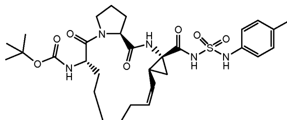
Compound 2243
