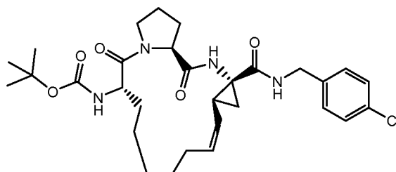
Compound 2308
