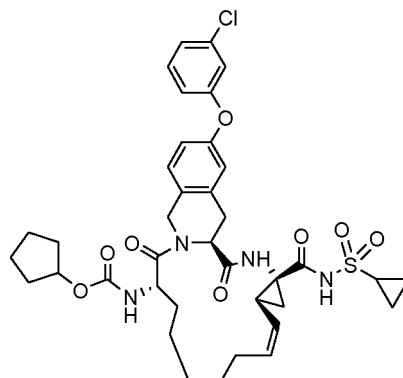
Compound 2005
