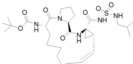
Compound 2218
