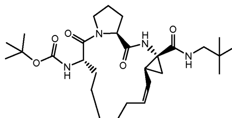
Compound 2315
