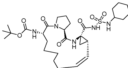
Compound 2205
