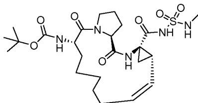
Compound 2213
