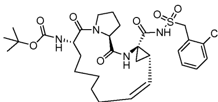
Compound 2117
