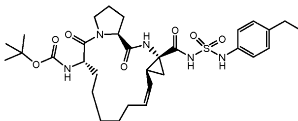
Compound 2242
