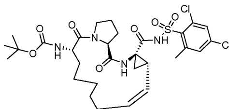
Compound 2123
