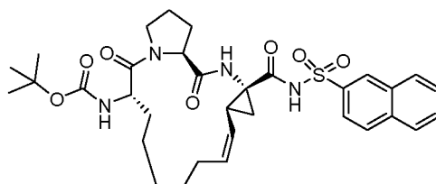
Compound 2130
