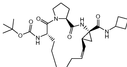
Compound 2303
