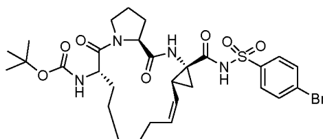
Compound 2131
