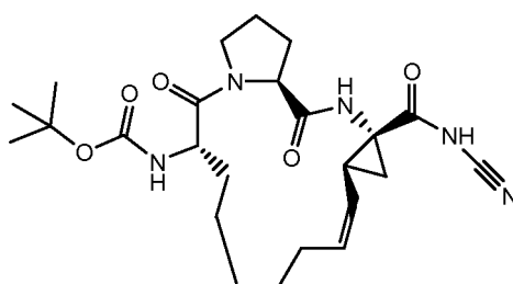
Compound 2306
