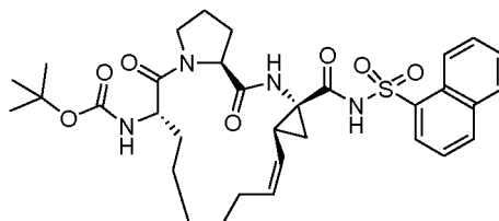
Compound 2148
