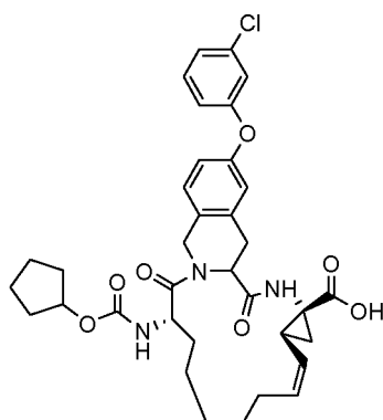
Compound 2002
