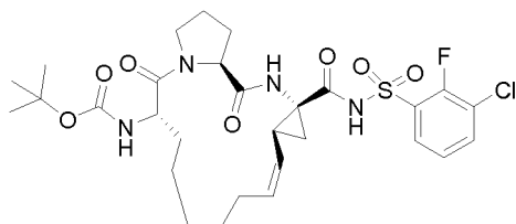
Compound 2151
