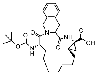
Compound 2011
