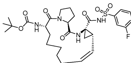
Compound 2113
