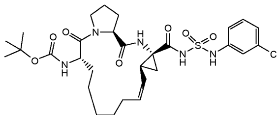
Compound 2239
