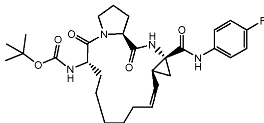
Compound 2304
