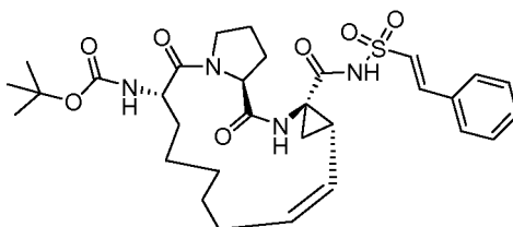
Compound 2125
