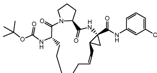
Compound 2317
