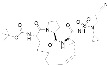
Compound 2210
