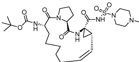
Compound 2208
