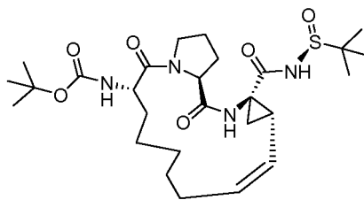
Compound 2401
