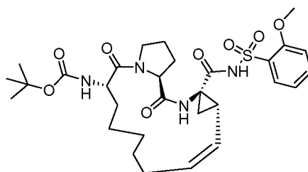
Compound 2122
