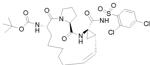
Compound 2153
