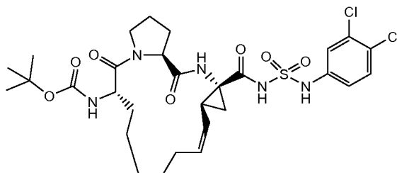
Compound 2234
