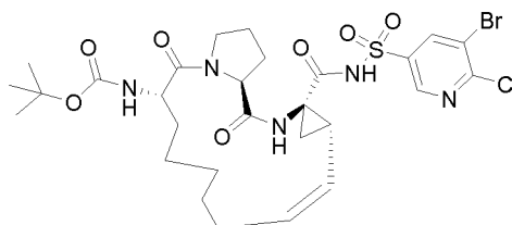
Compound 2154
