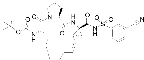
Compound 2152
