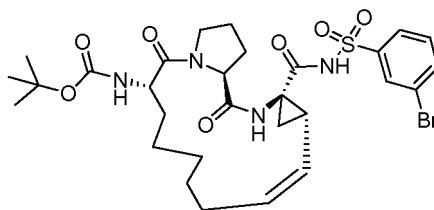
Compound 2112
