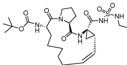
Compound 2216
