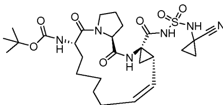
Compound 2212
