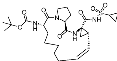
Compound 2137
