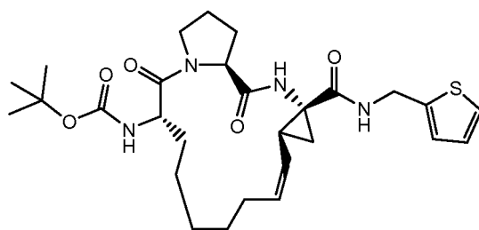
Compound 305
