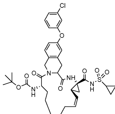
Compound 2007
