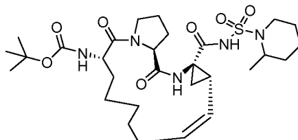
Compound 2225
