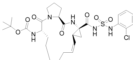
Compound 2233
