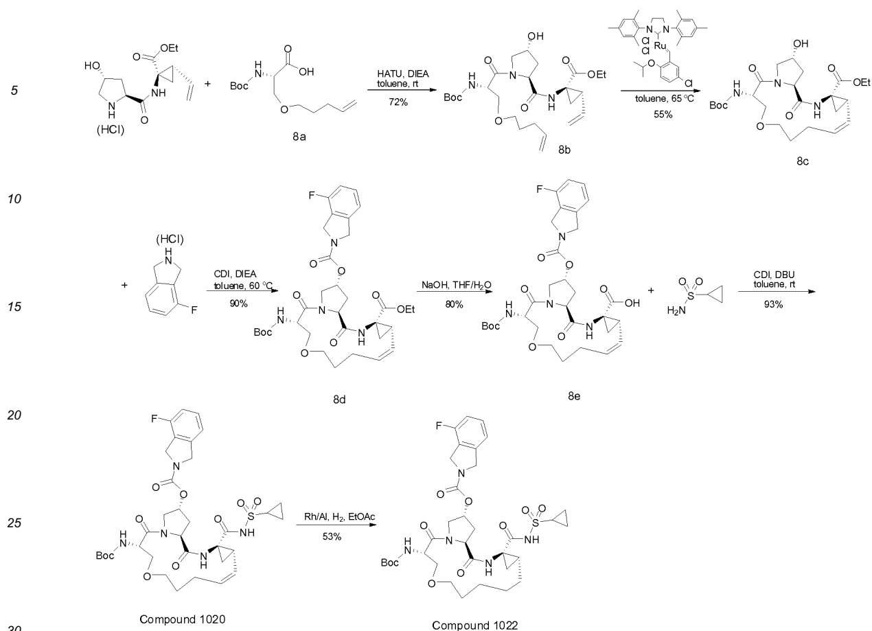
Scheme 8
