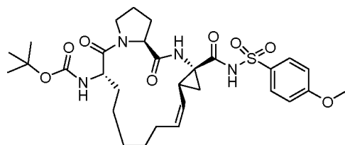
Compound 2133
