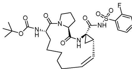
Compound 2124
