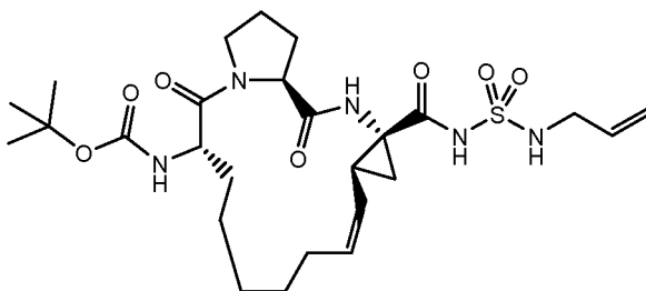
Compound 2238
