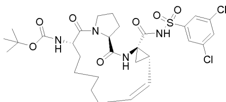
Compound 2108
