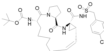
Compound 2119
