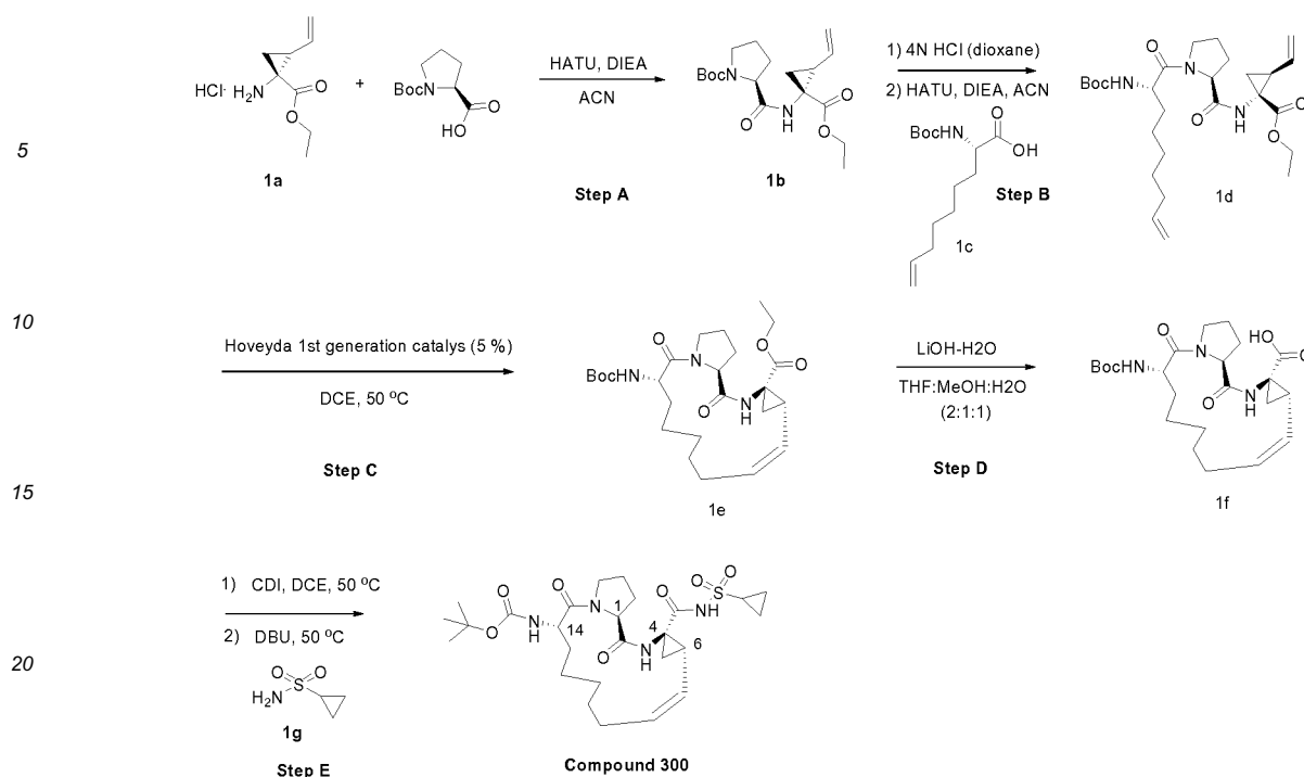
Scheme 4
