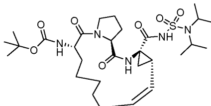
Compound 2209
