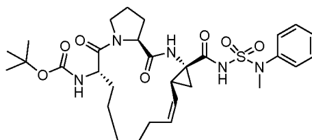
Compound 2227
