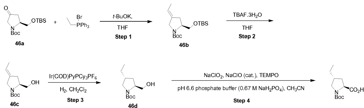
Scheme 14-4
