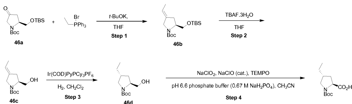
Scheme 4a
