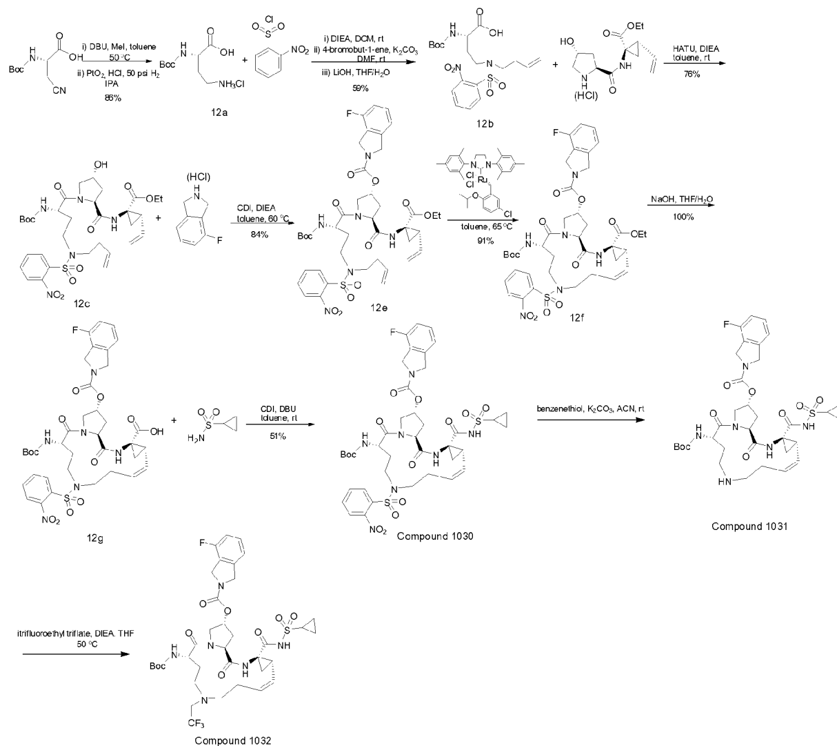
Scheme 12
