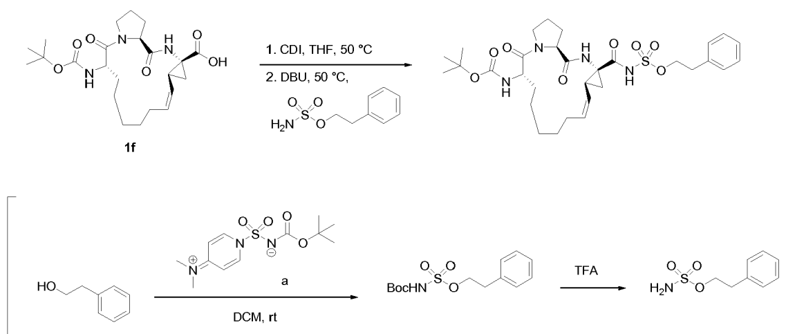
Scheme 6
