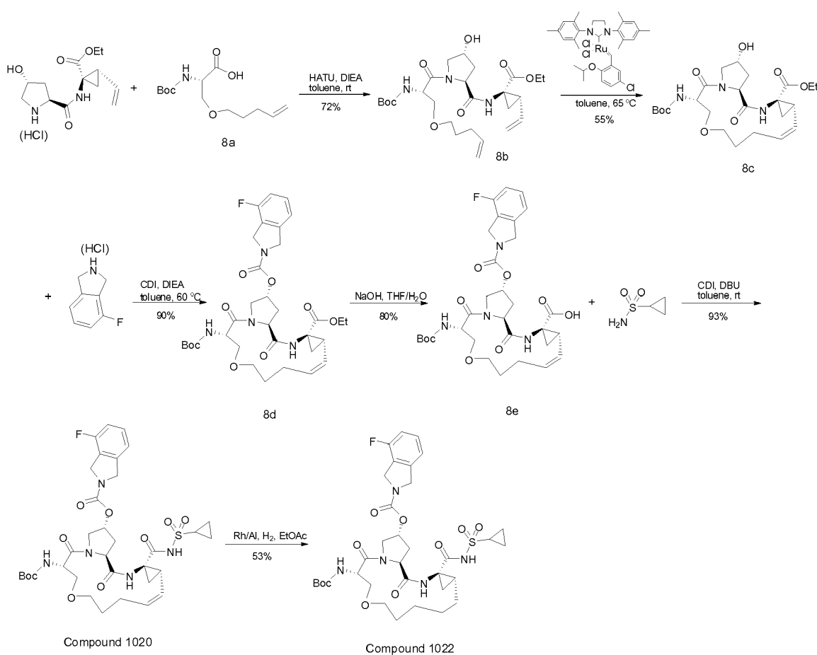
Scheme 8
