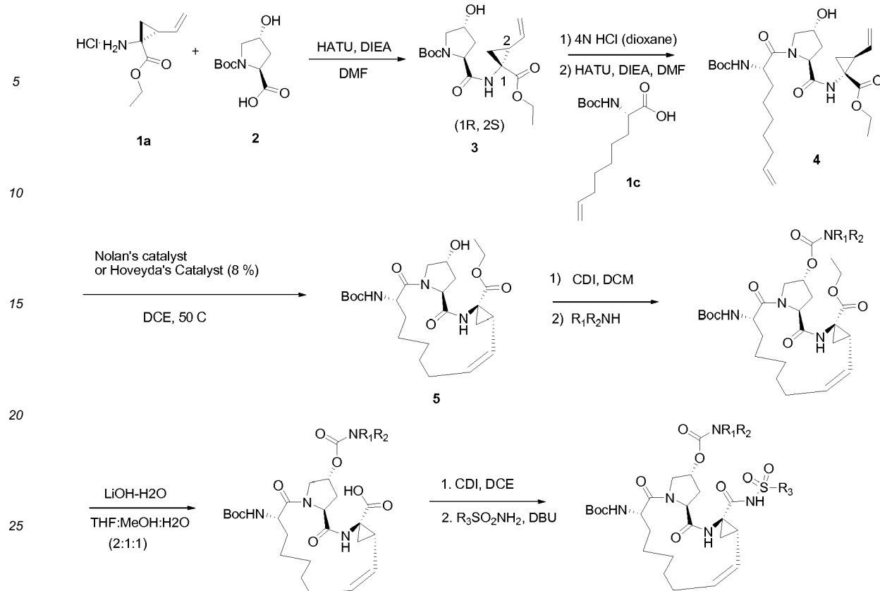
Scheme 1.
