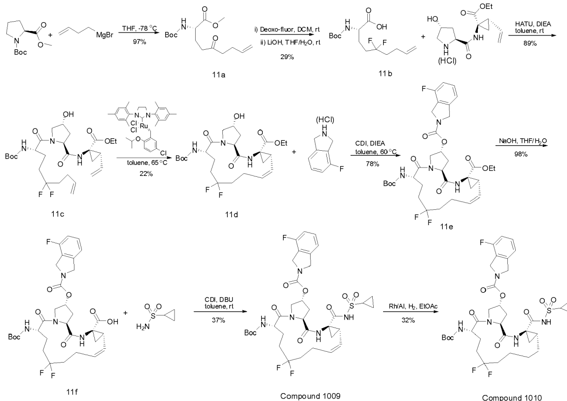
Scheme 11
