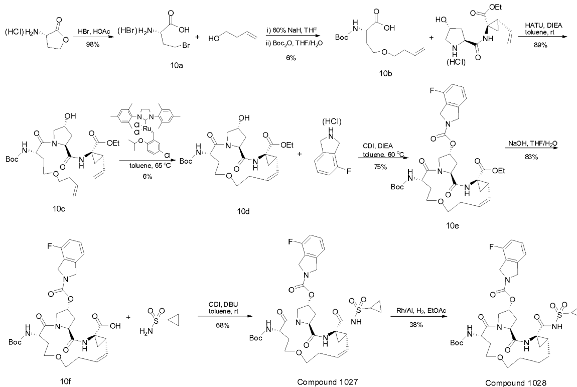
Scheme 10
