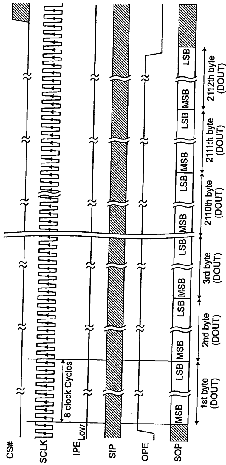
Basic Output Sequence in Byte Mode
