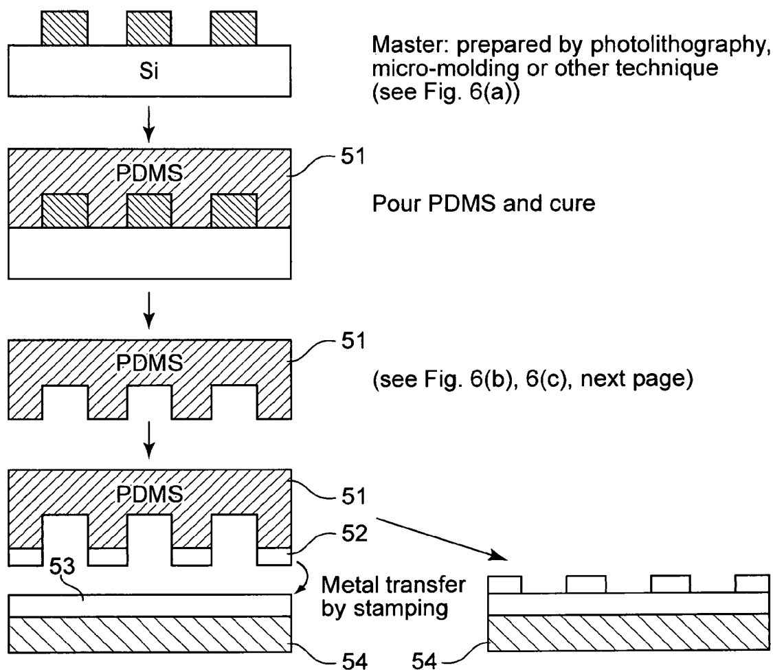
Fig. 5 Fabrication of PMDS stamp
