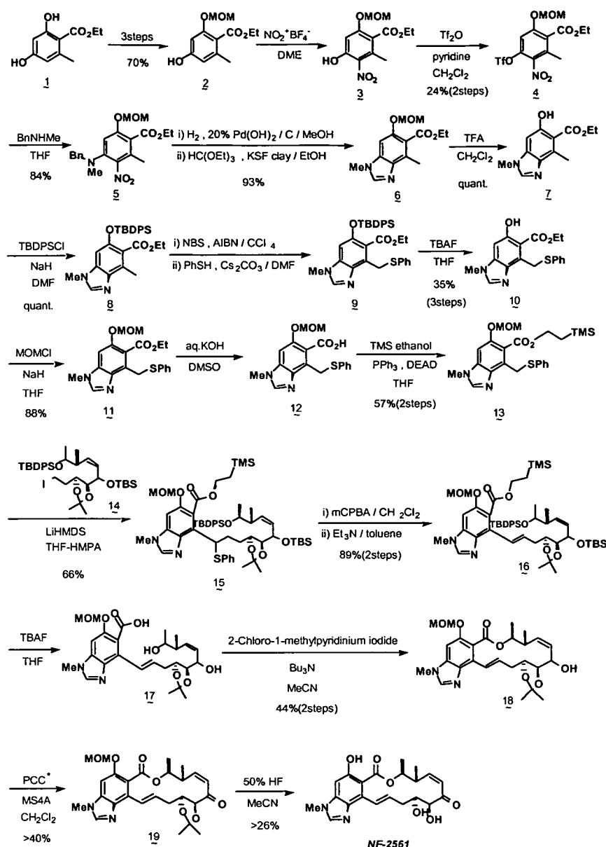
Scheme 10
