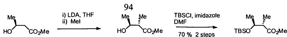
Methyl-3-hydroxybutyrate
