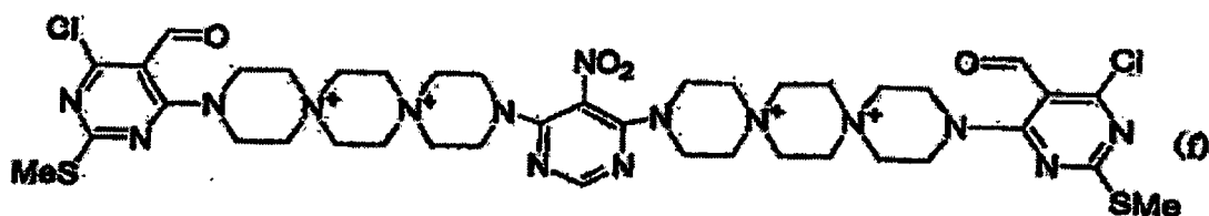
[Chem. 15]
