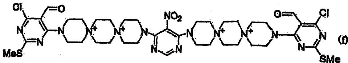
[Chem. 15]
