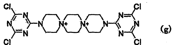
[Chem. 9]
