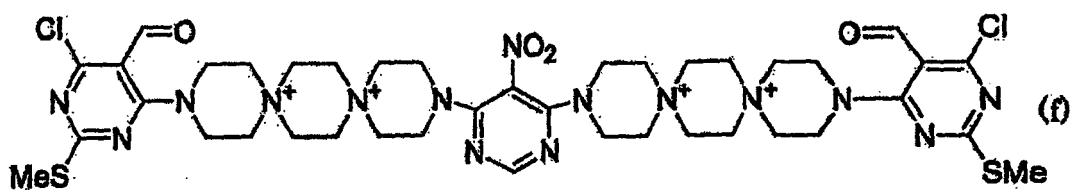
[Chem. 15]
