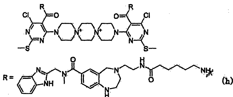
[Chem. 10]
