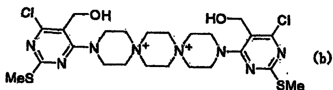
[Chem. 13]
