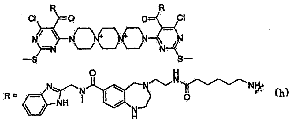
[Chem. 17]
