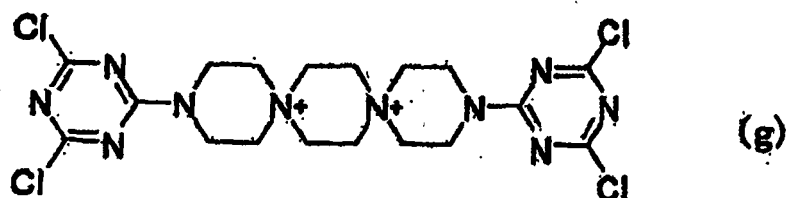
[Chem. 16]
