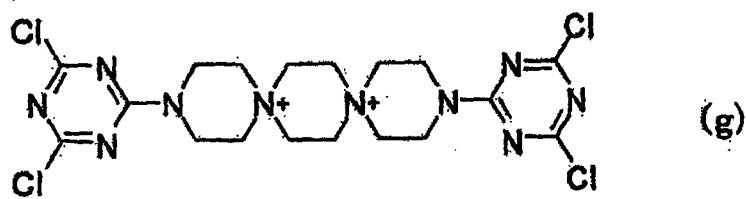
[Chem. 16]
