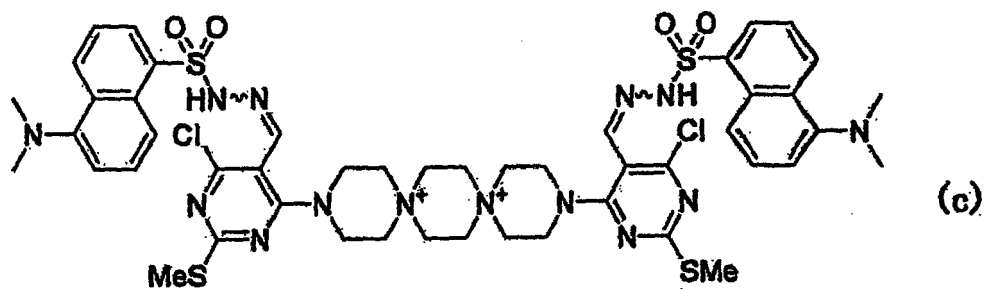
[Chem. 14]
