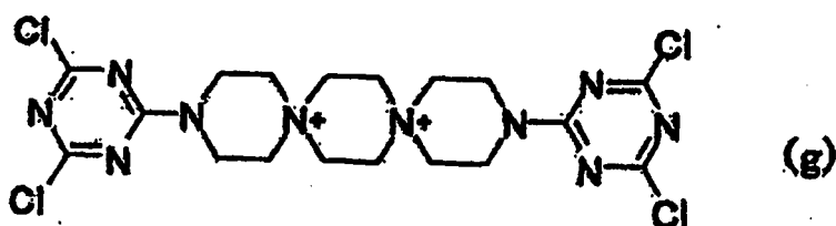
[Chem. 9]
