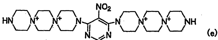
[Chem. 7]
