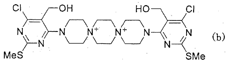
[Chem. 22]
