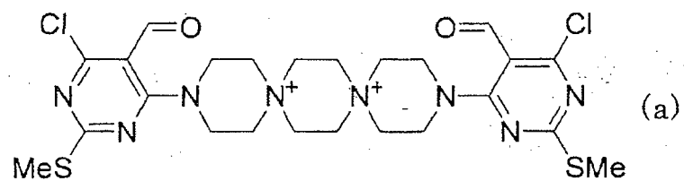
[Chem. 21]
