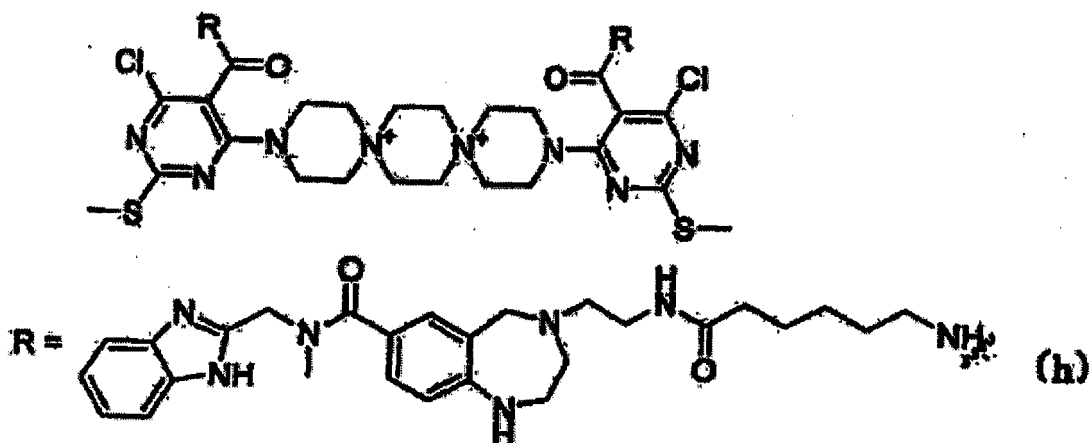
[Chem. 17]
