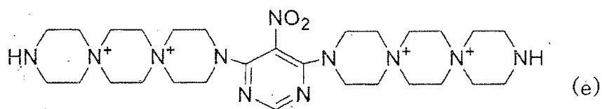
[Chem. 7]
