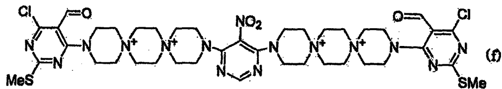
[Chem. 8]
