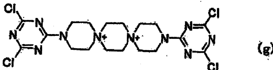
[Chem. 16]
