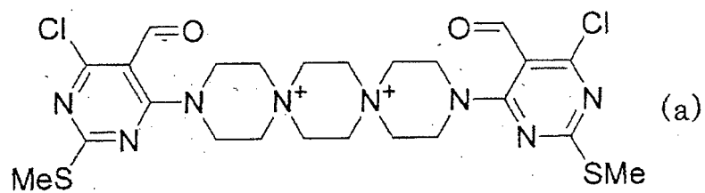
[Chem. 4]
