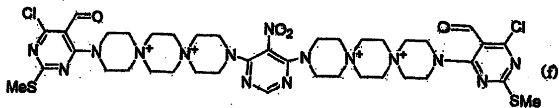
[Chem. 8]
