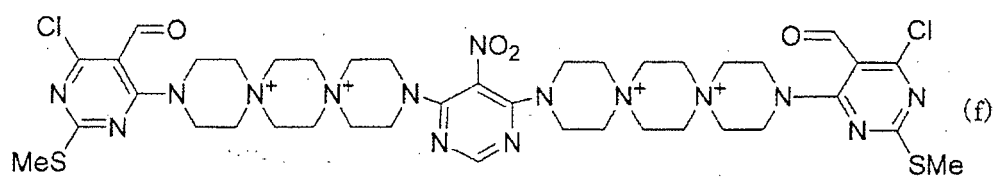
[Chem. 8]
