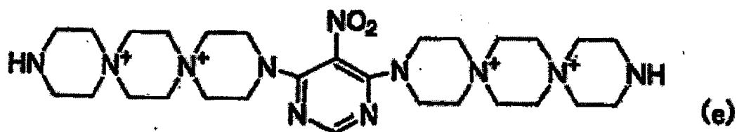
[Chem. 7]
