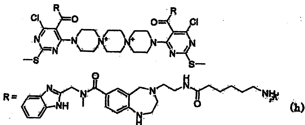
[Chem. 10]
