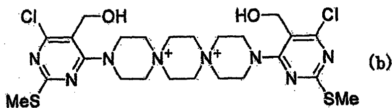
40 [Chem. 4]
