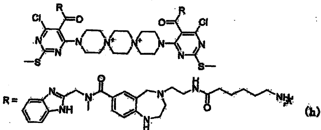
[Chem. 10]
