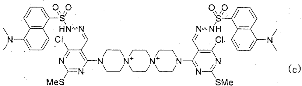
[Chem. 22]
