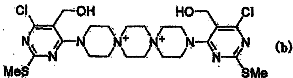
[Chem. 4]
