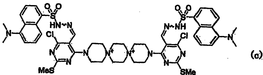
[Chem. 14]
