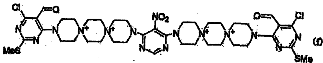
[Chem. 8]
