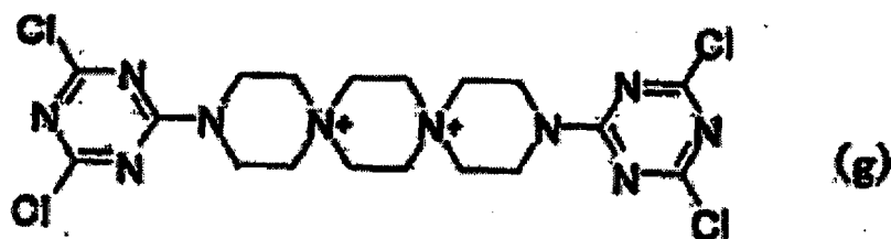
[Chem. 9]
