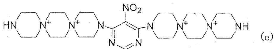
[Chem. 24]
