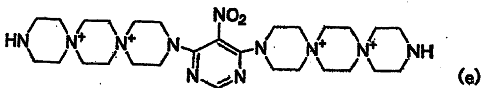
[Chem. 8]
