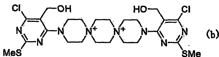
[Chem. 13]
