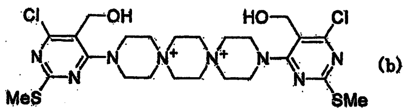
[Chem. 4]
