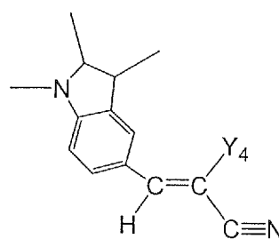
Z configuration
