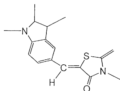
Z configuration
