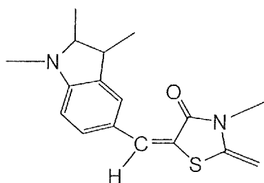
E configuration
