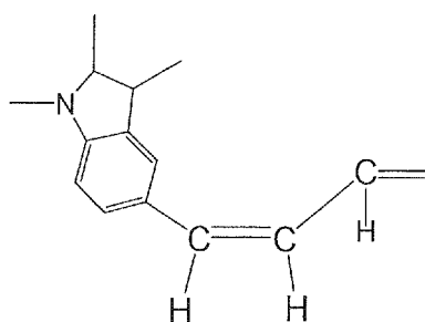
cis configuration
