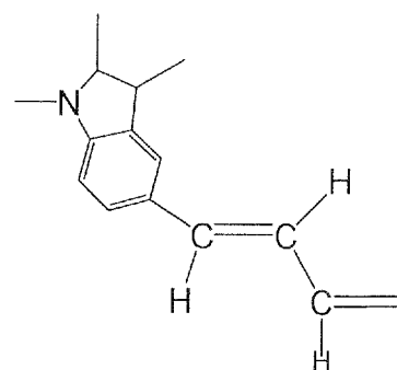
trans configuration
