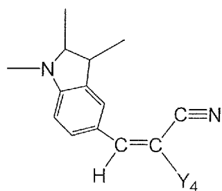
E configuration
