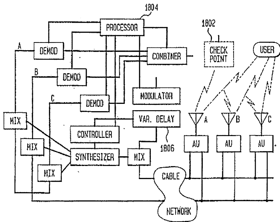
FIG. 18 TIME CALIBRATION FOR DISTRIBUTED ANTENNA IMPLEMENTATION
