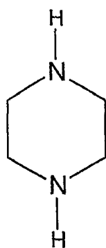
piperazine hydrogenated pyrazine
