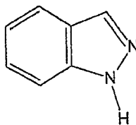
indazole
