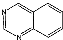
quinazoline
