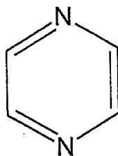
pyrazine
