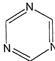
triazine
