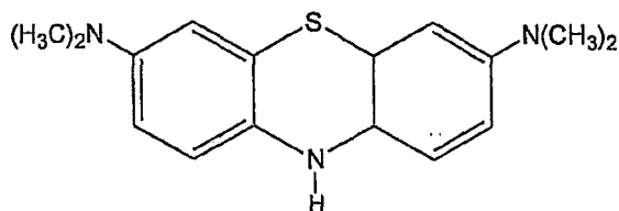
leucomethylene blue
