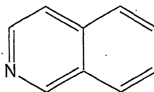
isoquinoline
