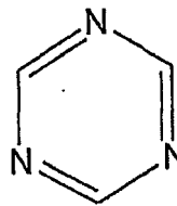
triazine
