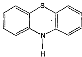
phenothiazine
