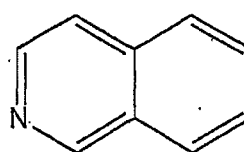
isoquinoline
