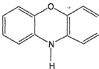
phenoxazine
