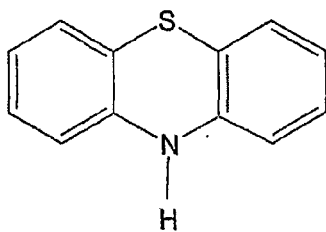
phenothiazine
