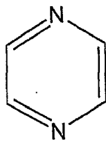
pyrazine
