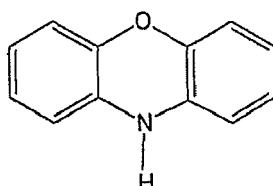
phenoxazine
