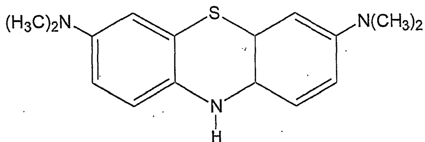
leucomethylene blue
