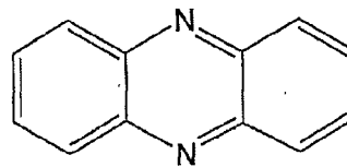
phenazine
