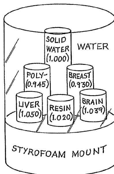
ELECTRON DENSITY PHANTHOM (CONTRAST, CT LINEARITY)
