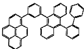
[Chem. 62]
