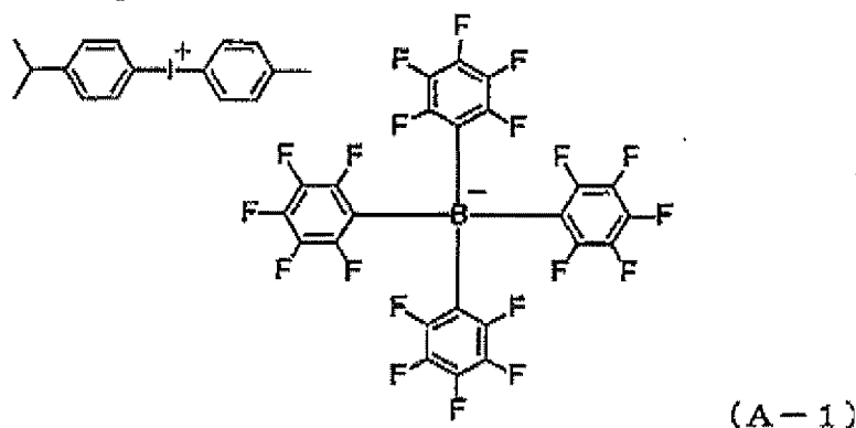
[Chem. 61]
