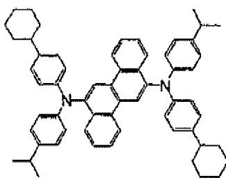
[Chem. 63]
