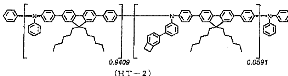
[Chem. 77]
