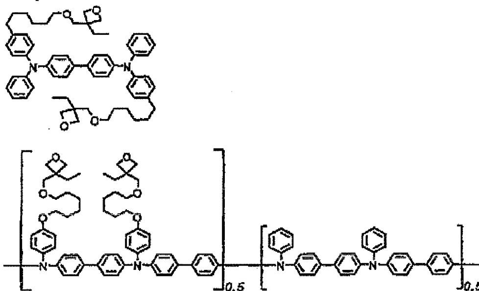
[Chem. 1]
