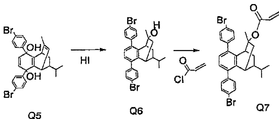
Scheme 4
