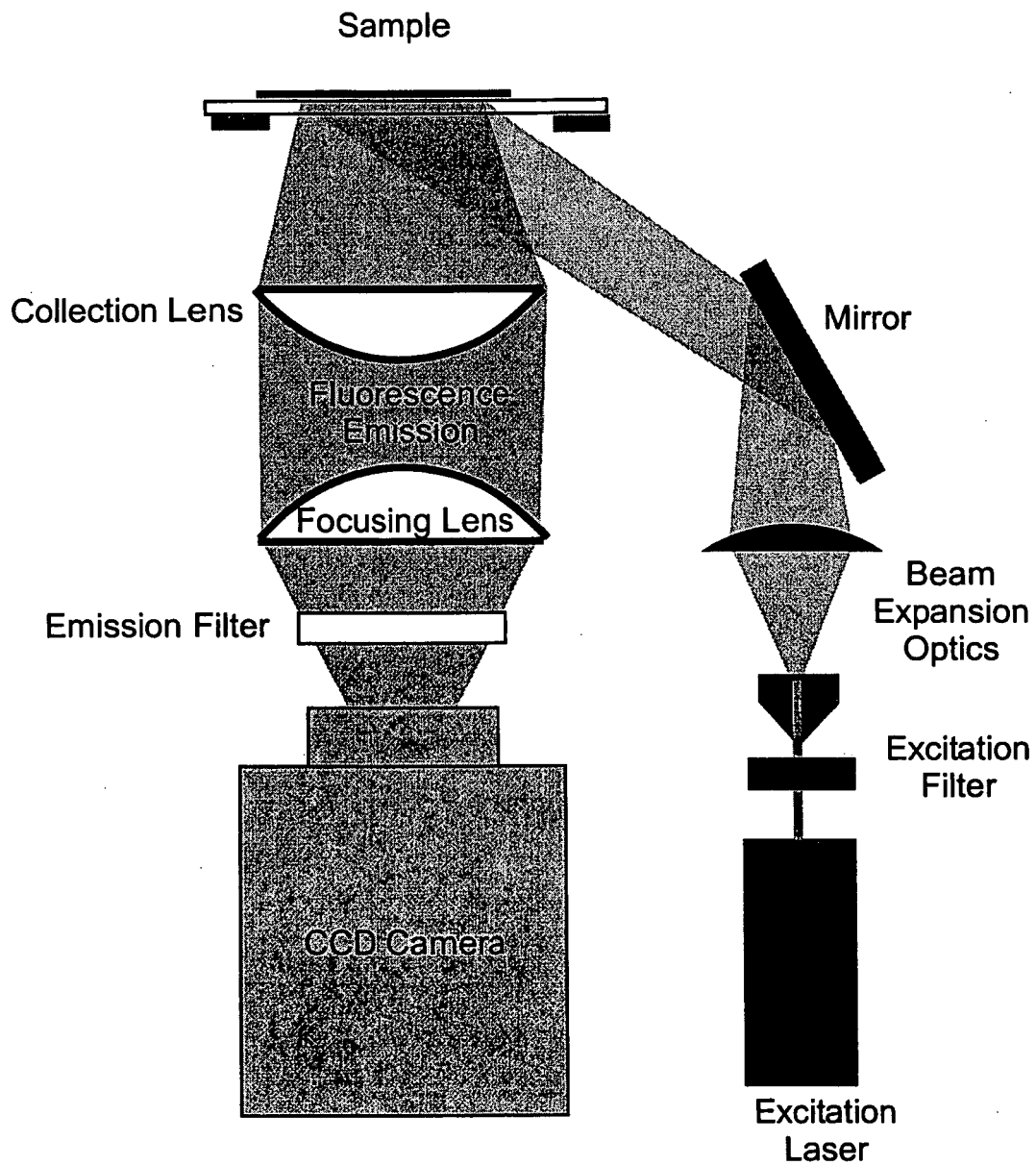
FIG. 4. A CCD imaging system for non-magnified large area imaging.
