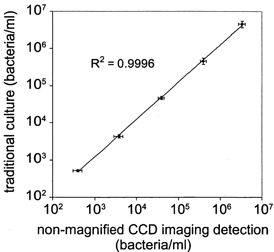
FIG. 12. Correlation between enumeration tests using the invention and traditional culture (Example 7).
