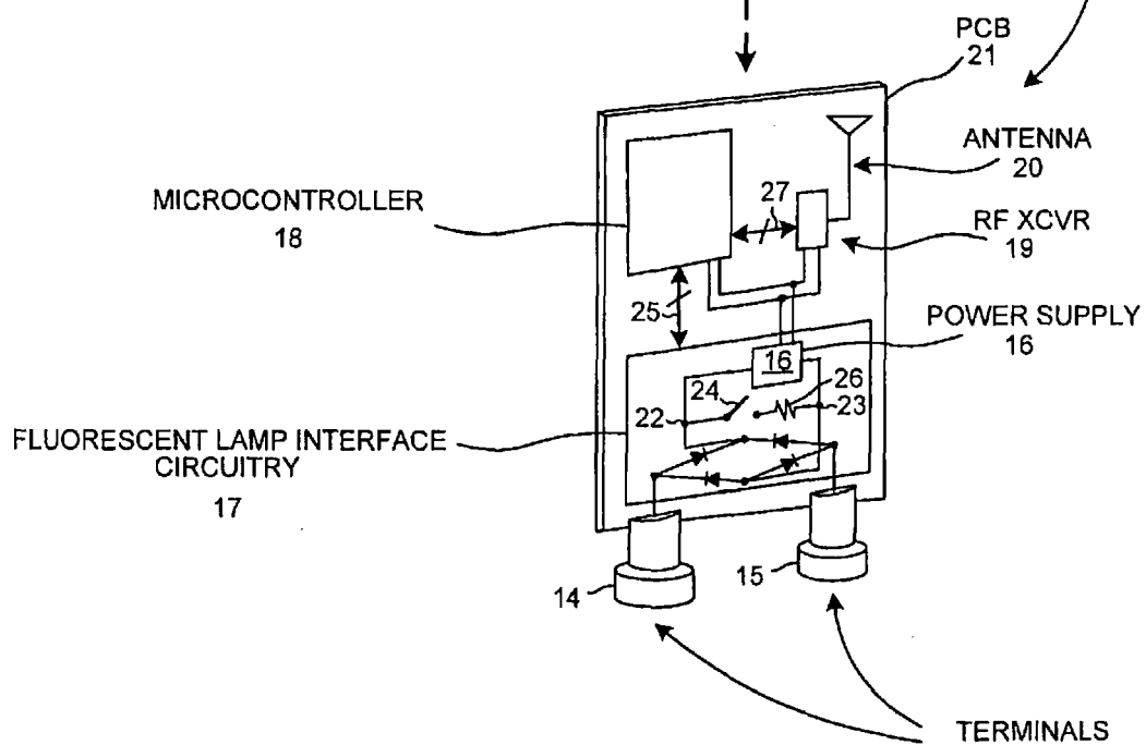
RF-ENABLED STARTER UNIT
