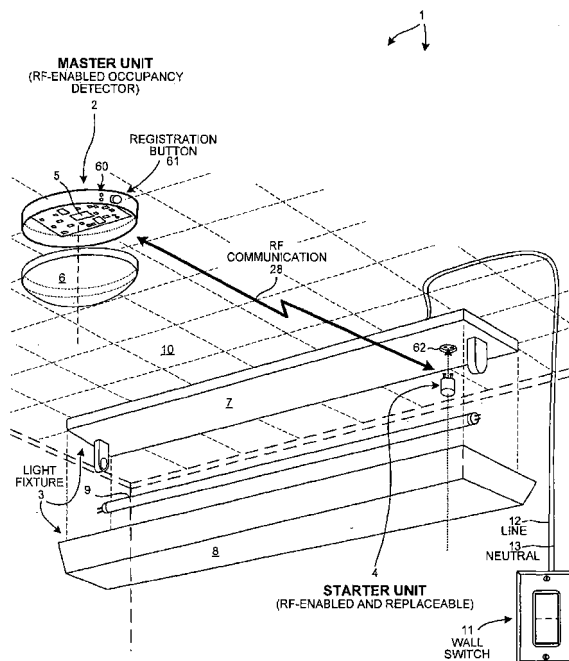
CENTRAL MASTER UNIT CONTROLS MULTIPLE LIGHT FIXTURES VIA RF-ENABLED STARTER UNITS
