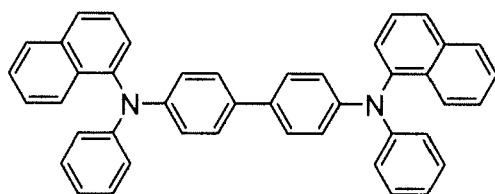
NPB
