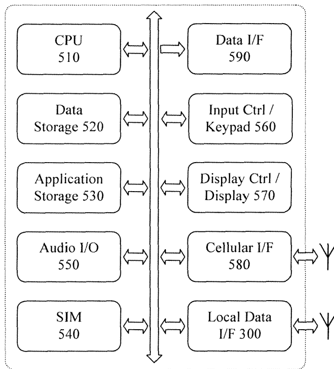
Portable CE Device 100
