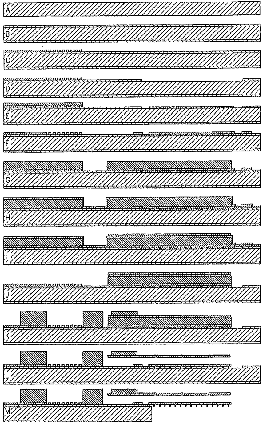
Silicon Pt/Ti Roughened Silicon Cr/Au Silicon Dioxide Photoresist Parylene SU-8
