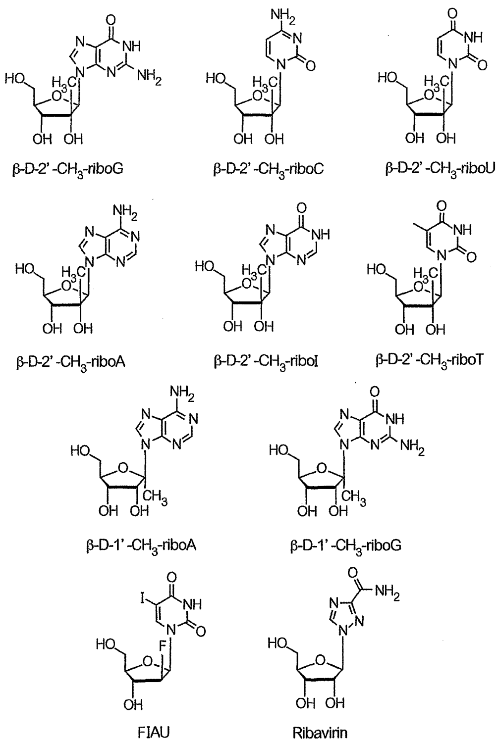
Chemical Structure of Illustrative Nucleosides
