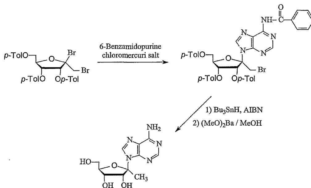
Scheme 7
