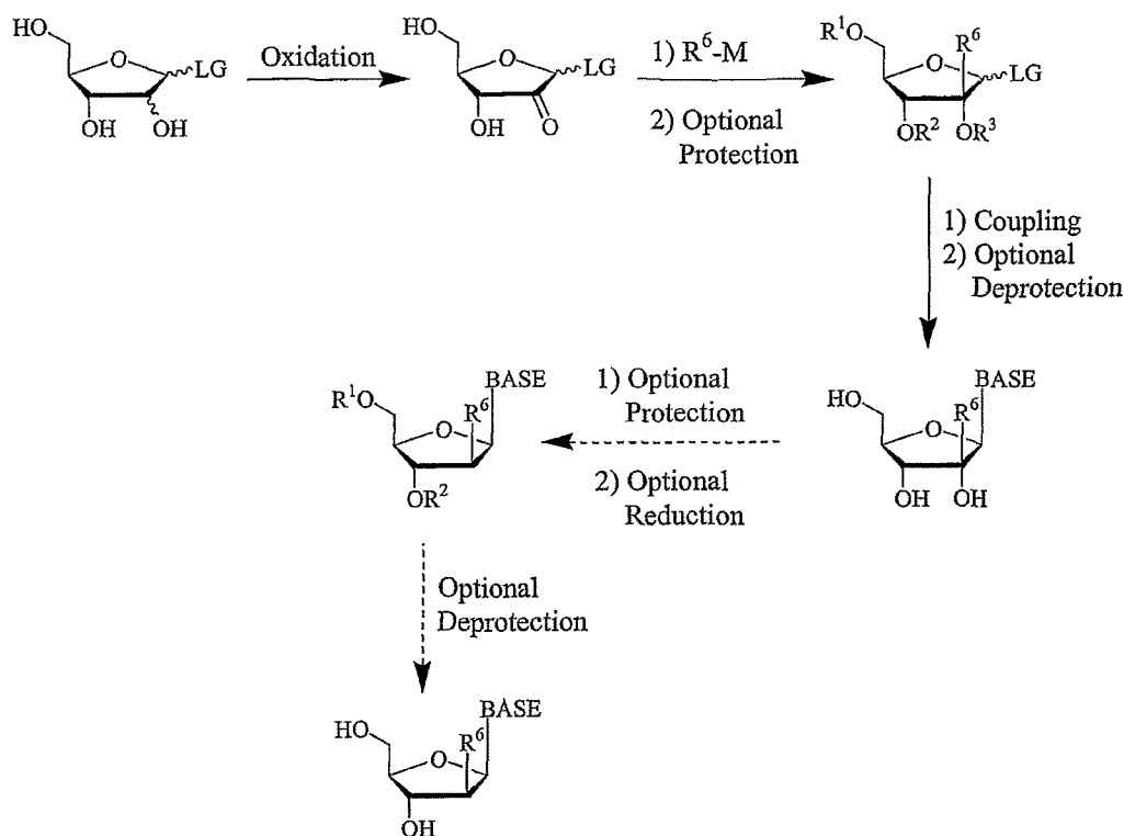
Scheme 3
