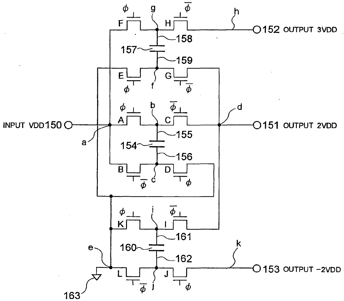
CHARGE-PUMP-TYPE VOLTAGE BOOSTING CIRCUIT
