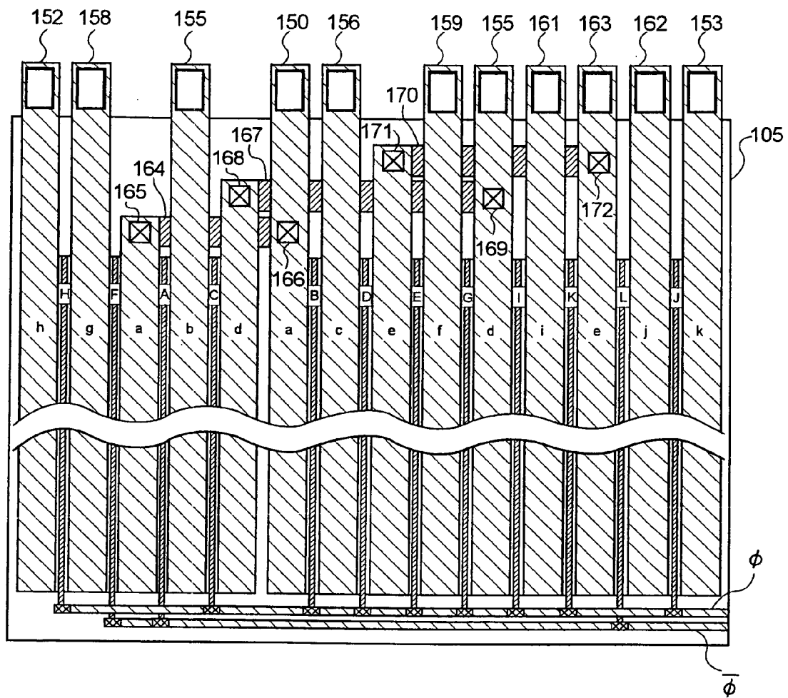
EXAMPLE OF AUTOMATIC LAYOUT
