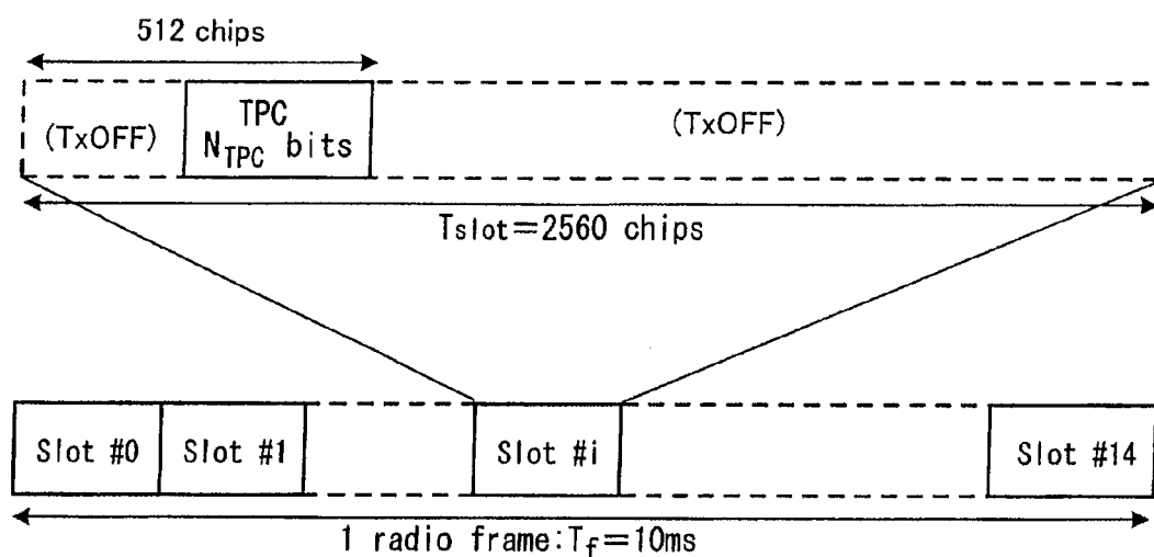
F-DPCH FRAME CONFIGURATION
