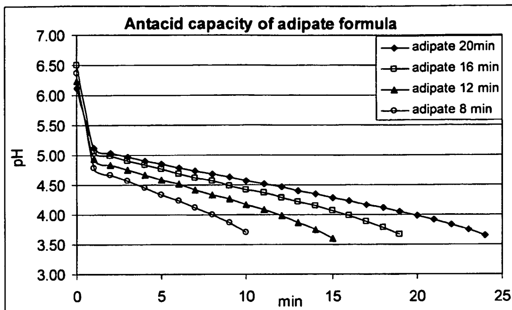
FIG. 2A Antacid capacity of various adipate formulations
