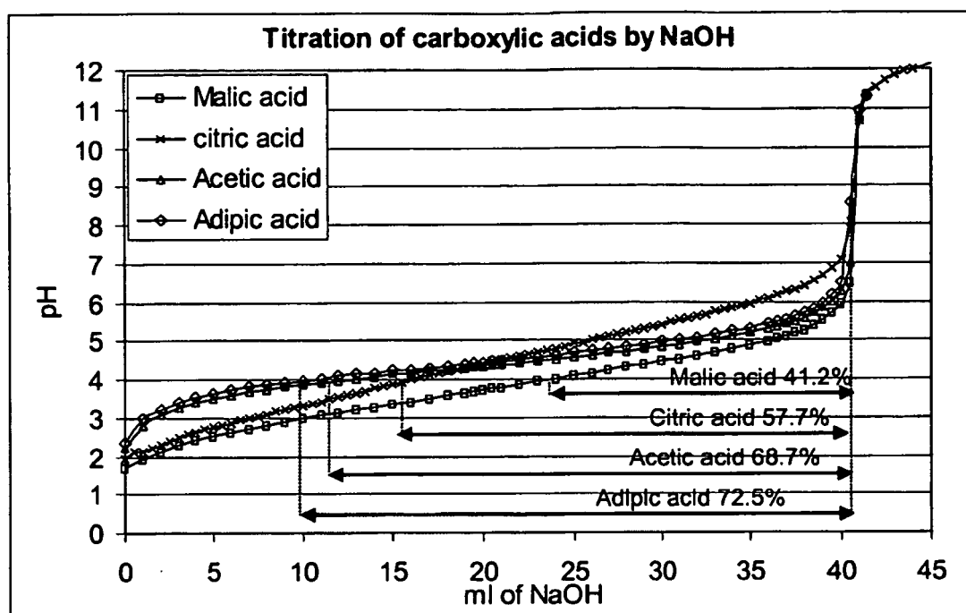
FIG. 1 Standard acid base titration curves of four carboxylates
