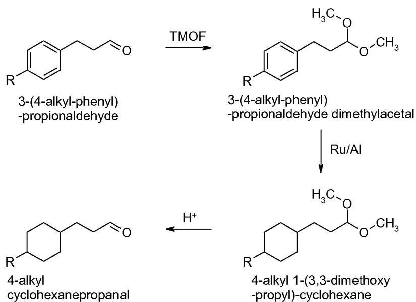
Scheme 2. Preparation of target compounds, 4-alkyl cyclohexanepropanals.
