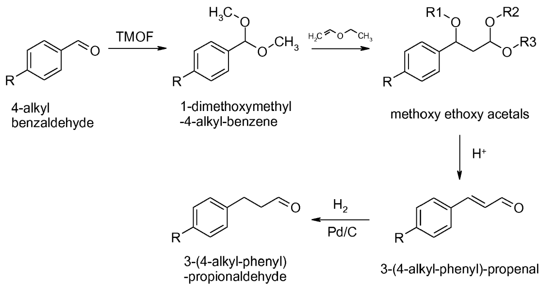
Scheme 1. Preparation of 3-(4-alkyl-phenyl)-propionaldehydes.
