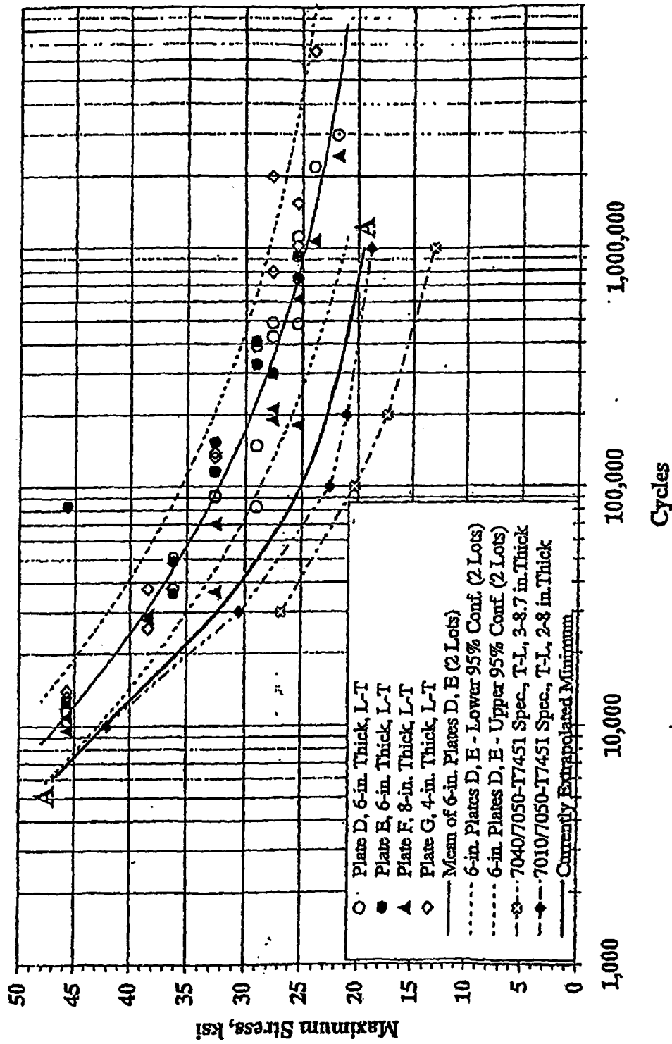
Figure 12 — Invention Alloy Plate Open-Hole S/N Fatigue for L-T Orientation K_t=2.3 , R=0.1 , \text{Freq.}=30 \text{ Hz} , \text{RH}>90\%
