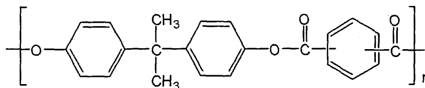
[Formula 2]
