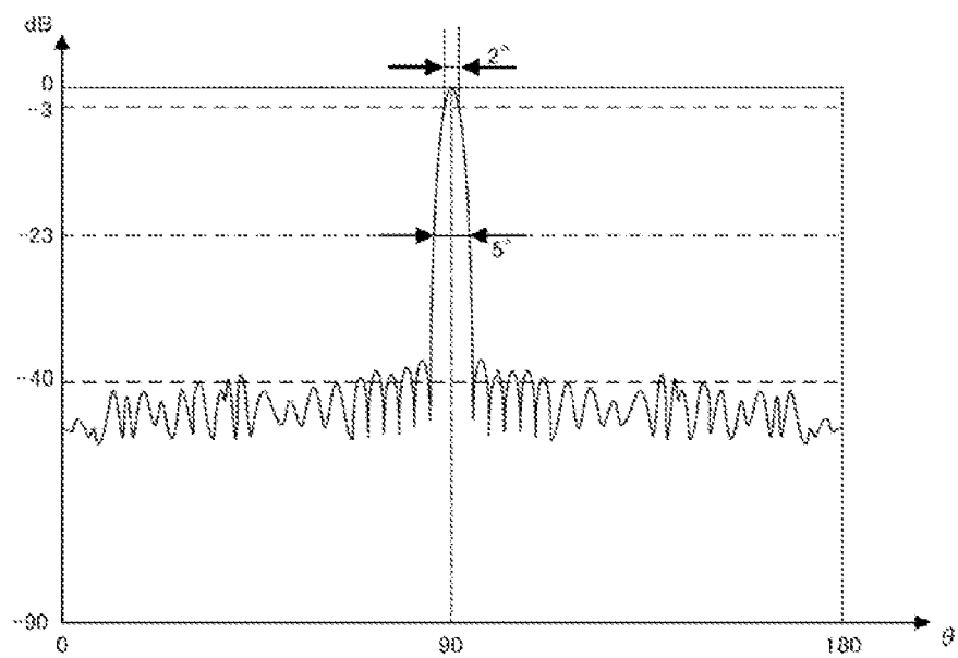
FIG. 2 (Related Art)
