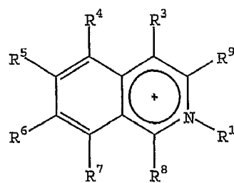
ISOQUINOLINIUM
