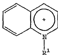
QUINOLINIUM
