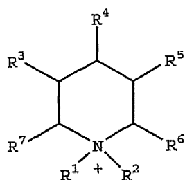
PIPERIDINIUM
