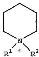
PIPERIDINIUM
