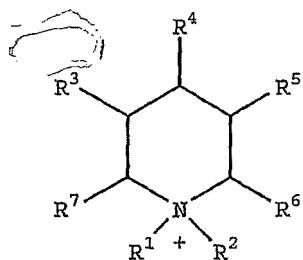
PIPERIDINIUM
