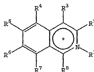
ISOQUINOLINIUM
