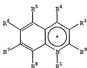
QUINOLINIUM
