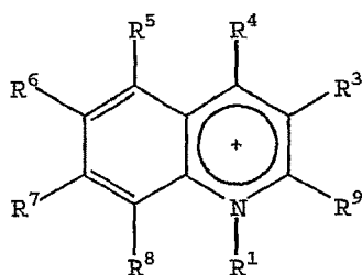
QUINOLINIUM
