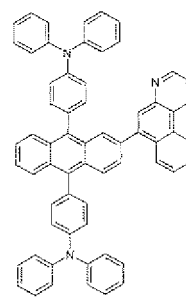
[Formula 3-12]
