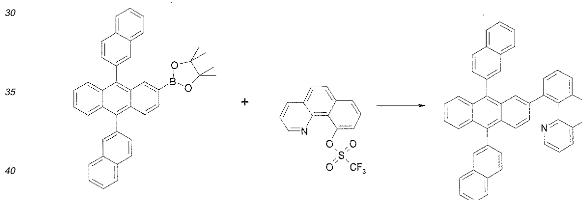
[Formula 1-82]
