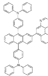
[Formula 3-12]
