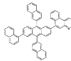
[Formula 3-36]
