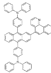
[Formula 1-52]
