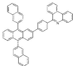
[Formula 2-17]
