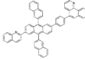
[Formula 1-79]
