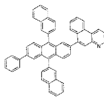
[Formula 3-35]
