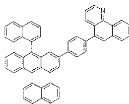
[Formula 1-62]
