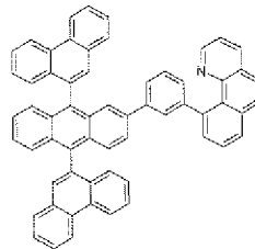
[Formula 1-103]
