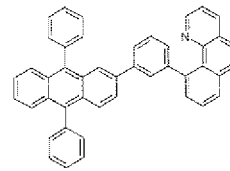
[Formula 1-104]
