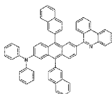
[Formula 2-37]
