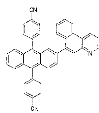
[Formula 3-32]
