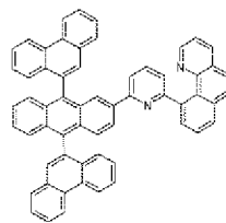
[Formula 1-107]
