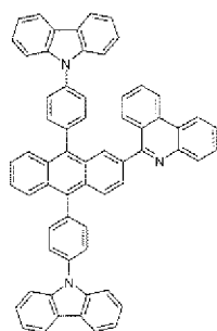
[Formula 2-9]
