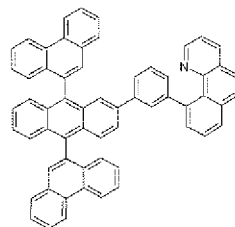
[Formula 1-103]
