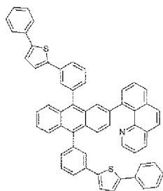
[Formula 1-93]
