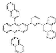
[Formula 3-25]
