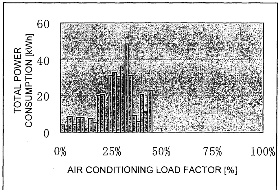
TOTAL POWER CONSUMPTION FOR EACH AIR CONDITIONING LOAD FACTOR (COOLING OPERATION)
