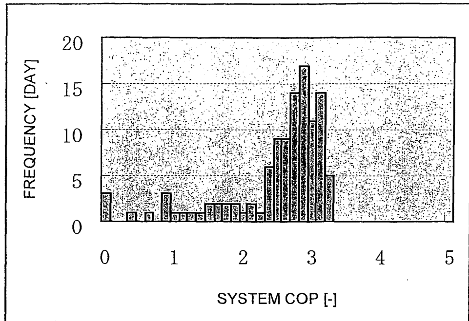
BAR CHART OF SYSTEM COP (COOLING OPERATION)
