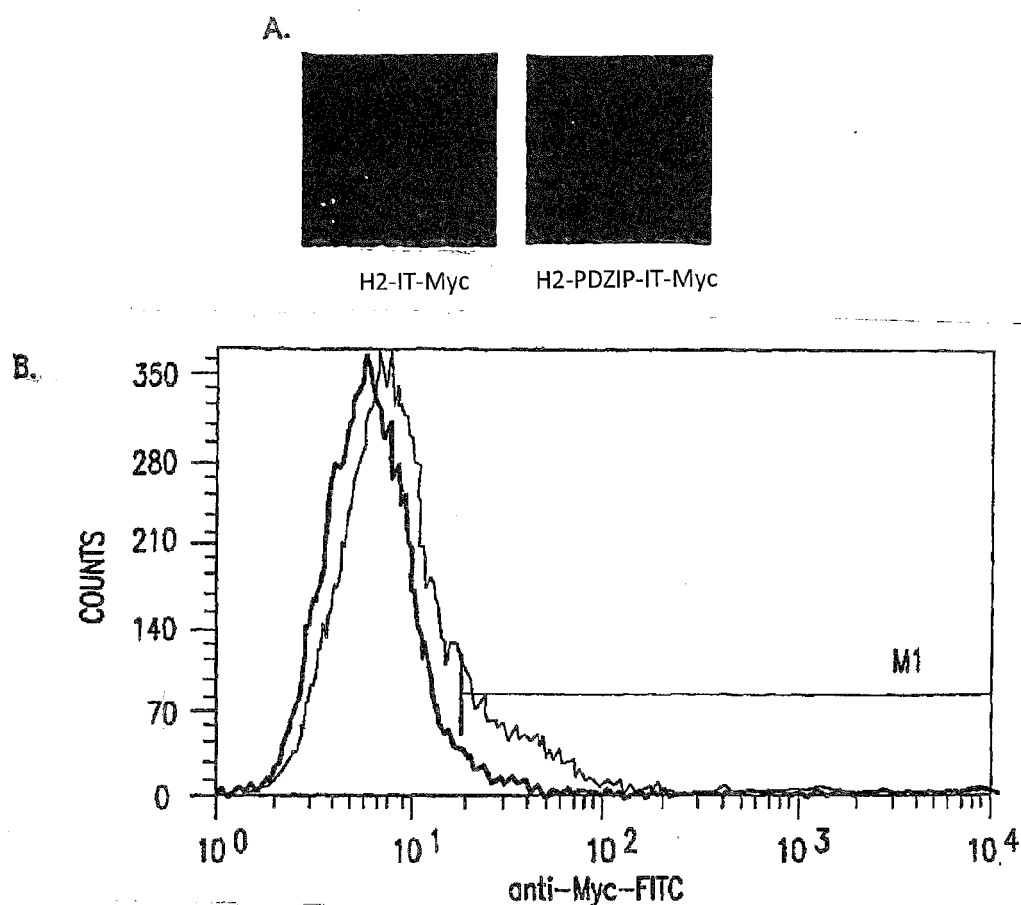
Figure 9 PDZIP facilitate the surface expression of human T1R2.
