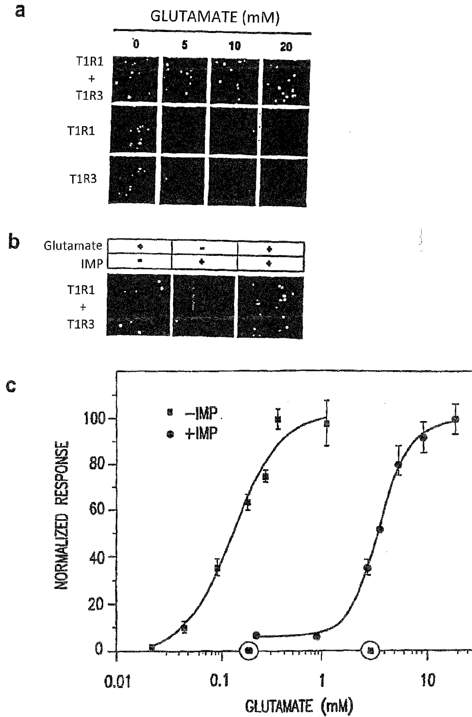
Figure 8 Human T1R1/T1R3 functions as an umami taste receptor
