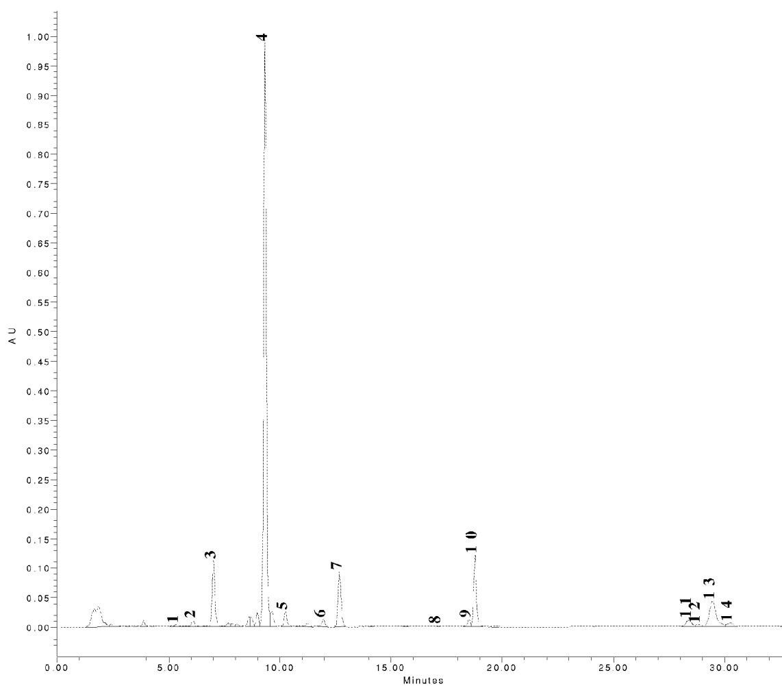
Figure 1. Representative HPLC chromatogram of saponified ground Capsicum from Example 8.
