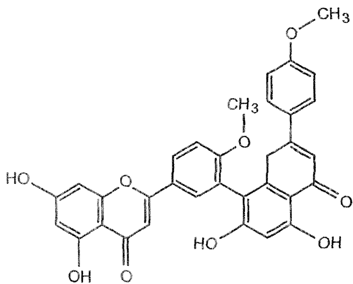
2-{3-[2,4-Dihydroxy-7-(4-methoxy-phenyl)-5-oxo-5, 8-dihydro-napthalen-1-yl]-4-methoxy-phenyl} -5,7-dihydroxy-chromen-4-one
