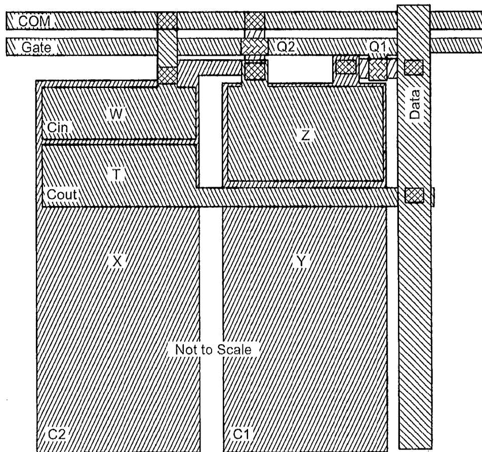
Subpixel Layout
