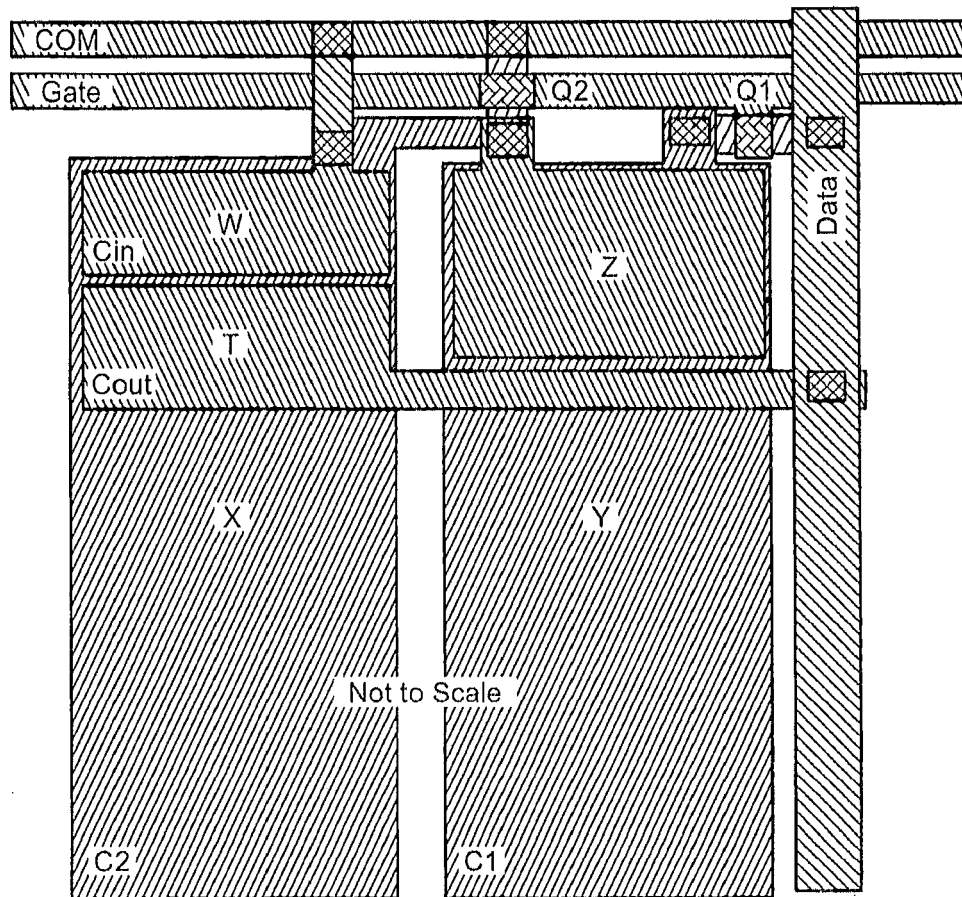
Subpixel Layout
