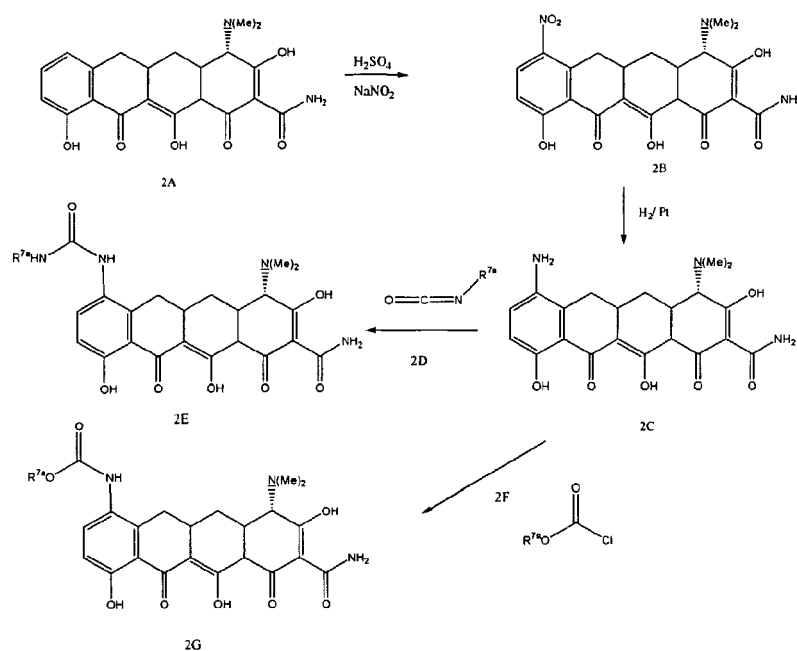
SCHEME 2
