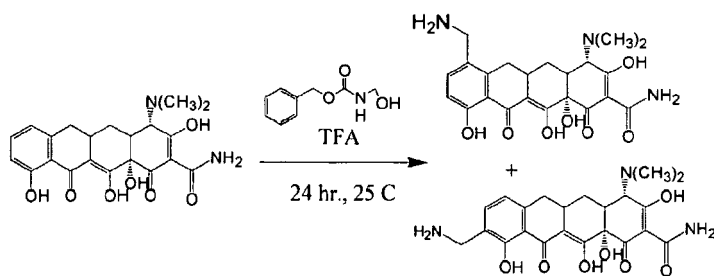
SCHEME 10
