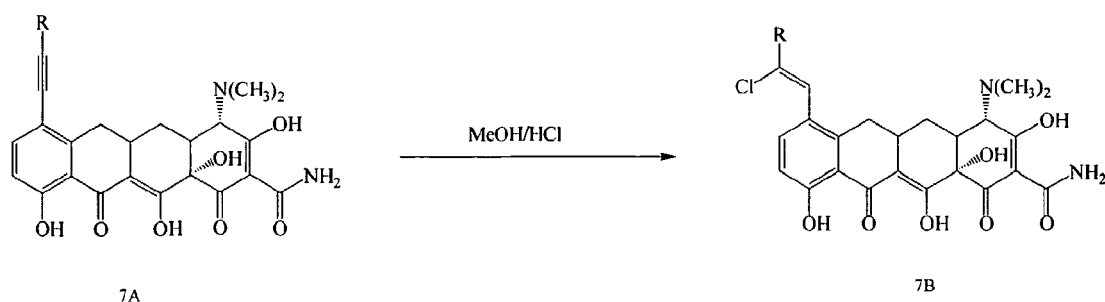
SCHEME 7
