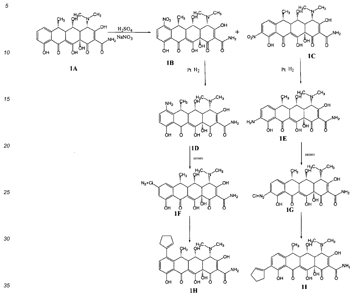
SCHEME 1
