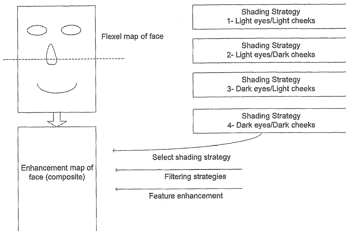
FIG. 43 - Example Artistic Strategy
