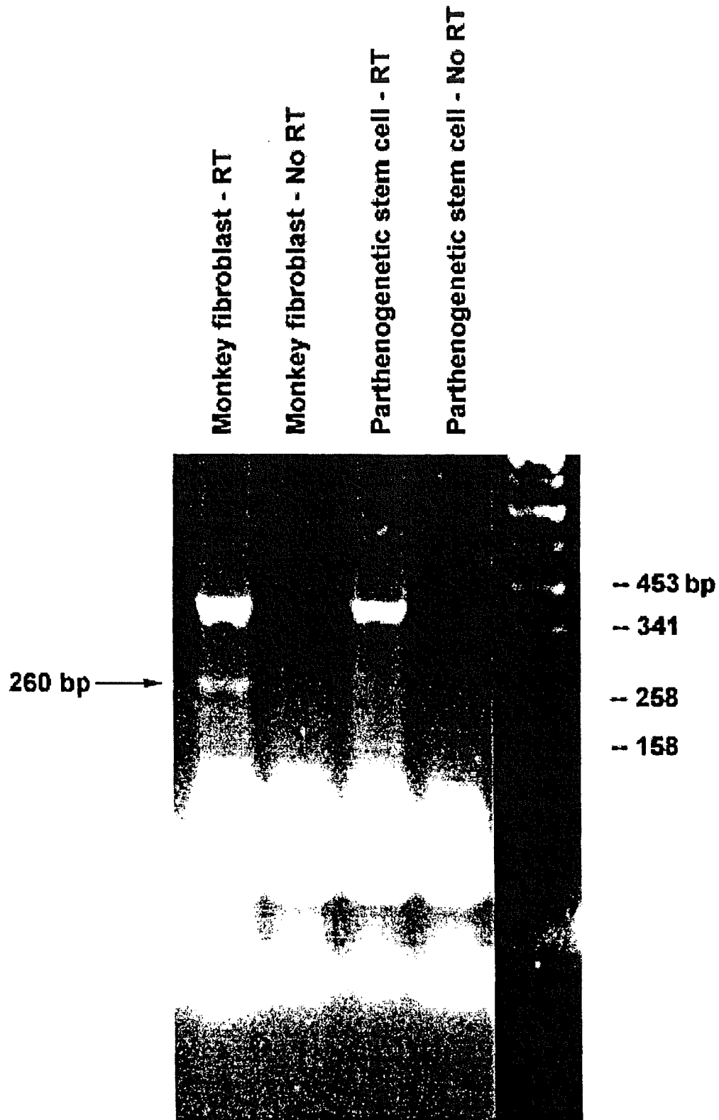
Figure 17. RT-PCR for snrpn in PPSCs.
