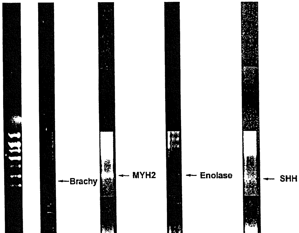
Figure 16. RT-PCR results demonstrating differentiation of multiple somatic cell types in differentiating PPSCs. Brachy: Brachyury (T) protein, MYH2: Skeletal myosin Heavy Polypeptide 2, Enolase: Human neuron-specific Enolase 2, SHH: Human homolog of Sonic Hedgehog.
