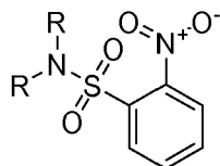
Scheme 4.2 Ns (2-Nitro-benzenesulfonyl) protection group used for protection of secondary amines.
