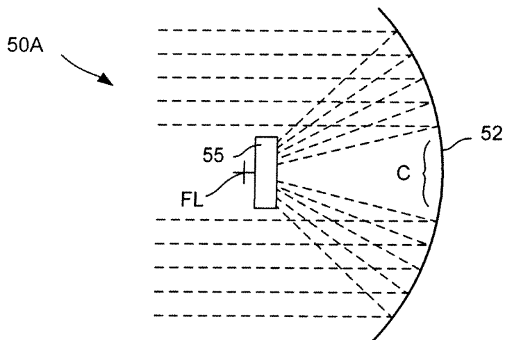
FIG. 18(B) (PRIOR ART)
