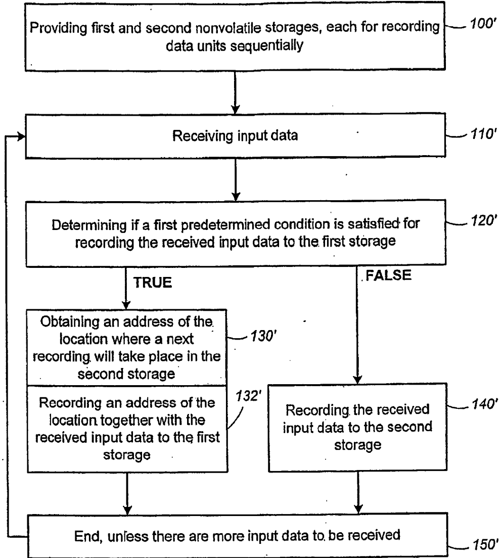
Synchronizing Two Update Streams Using Write Pointers
