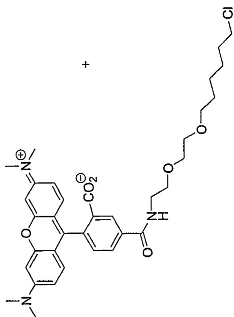
a compound of formula VIII
