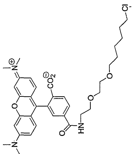
a compound of formula IX
