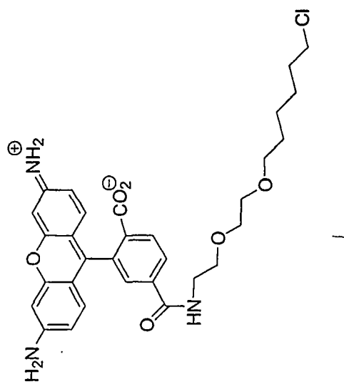
a compound of formula XI
