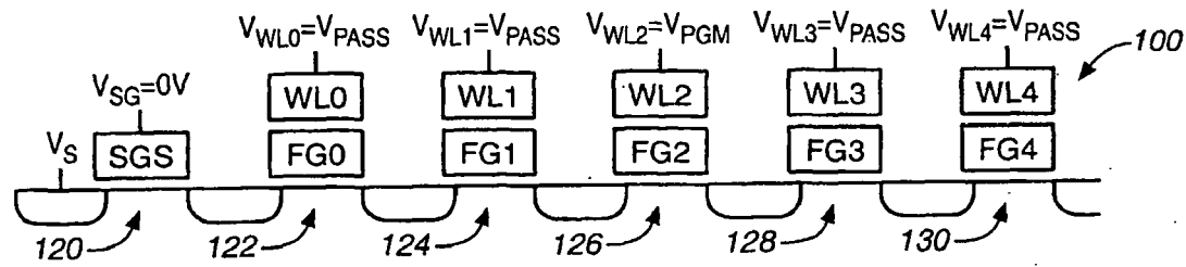
FIG. 4C (PRIOR ART)
