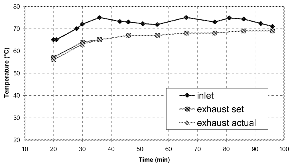
Curing of Example 14.1 Temperature Profile
