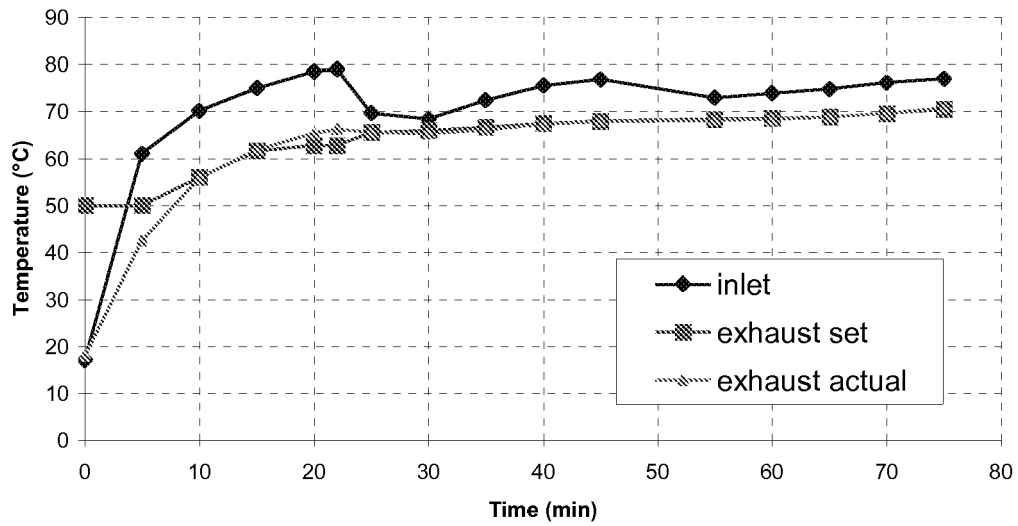
Curing of Example 14.3 Temperature Profile
