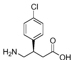
Baclofen-(a)
