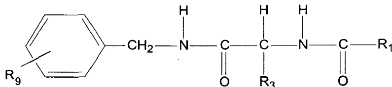
Formula (III)
