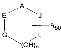
Formula (IV)
