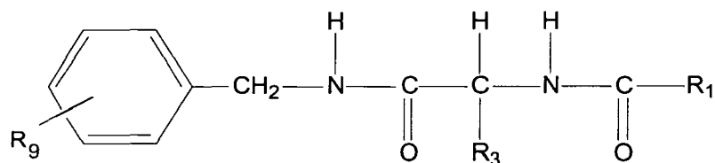
Formula (III)
