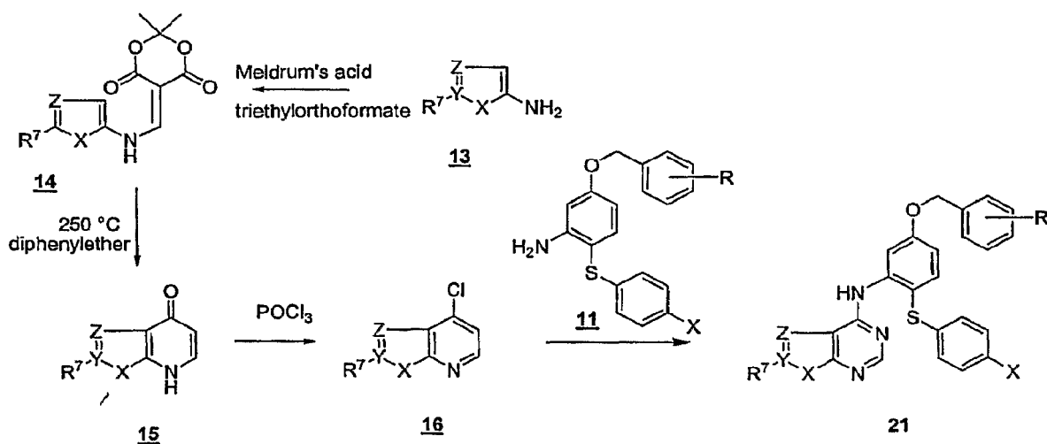
Scheme 7
