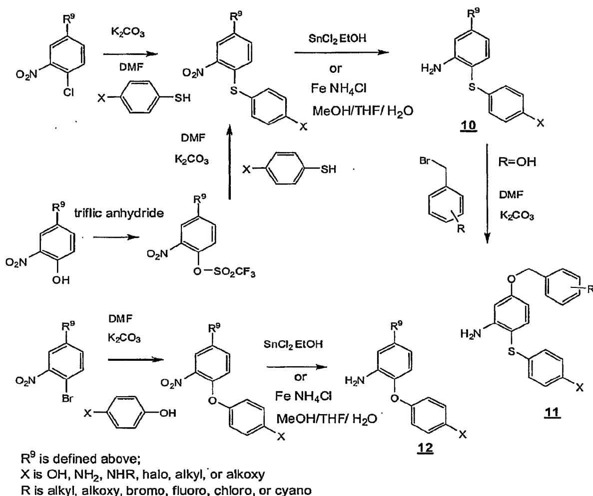
Scheme 4
