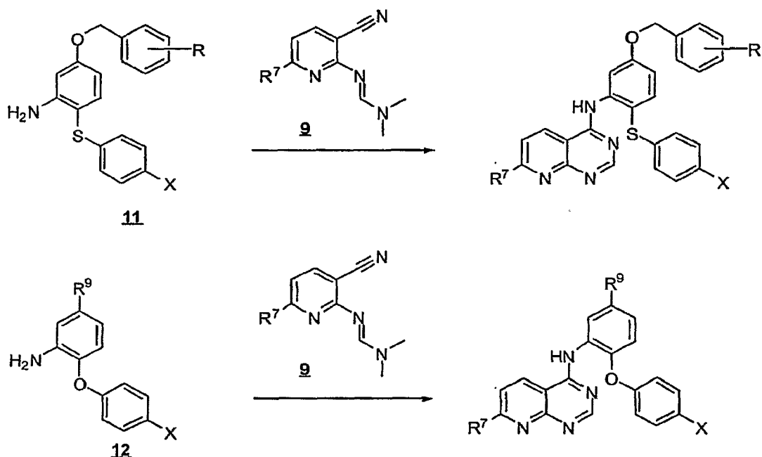
Scheme 6
