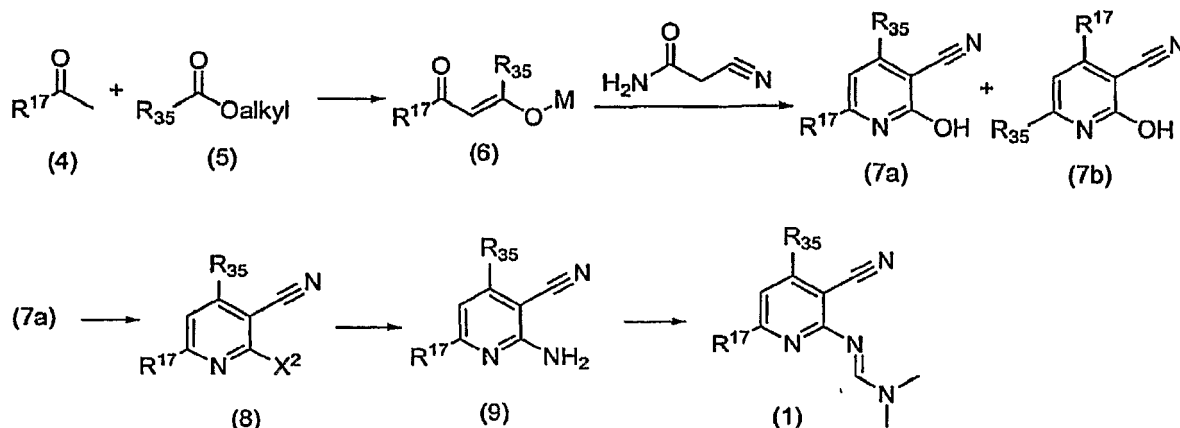
Scheme 2
